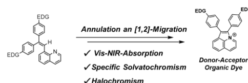
Scheme 2. Synthesis of D-A Type Dye with Cationic Aza-doped Acenaphthylene
