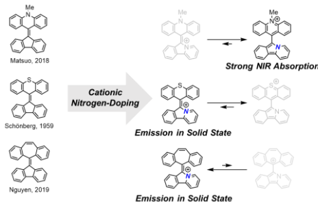
Scheme 3. Cationic Nitrogen-Doping into BAEs
