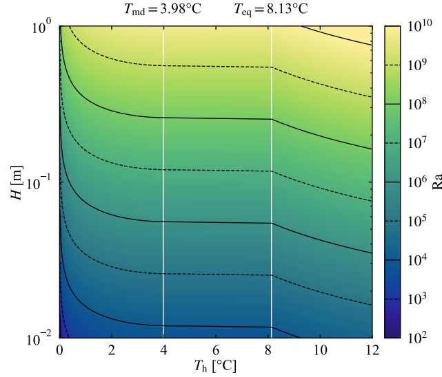
FIG. 9. Rayleigh number of ice-bounded coldwater convection.
