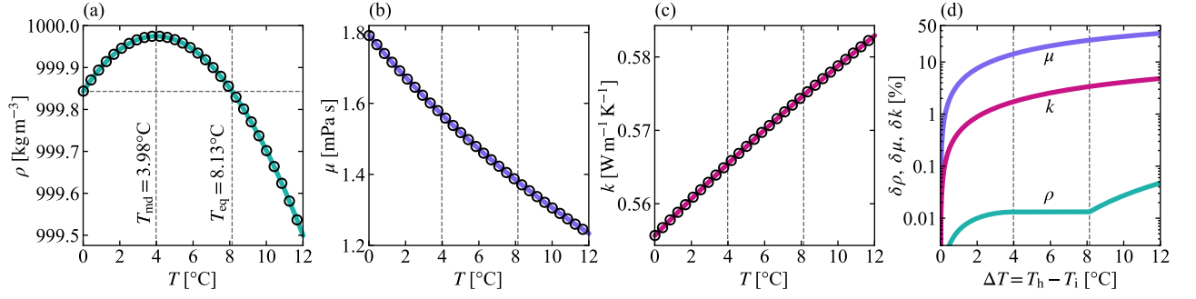
FIG. 2. Temperature-dependent material properties: (a) Density \rho(T) , (b) dynamics viscosity \mu(T) , and (c) thermal conductivity k(T) . Scatter plots are thermophysical properties database from NIST [37], and solid lines are the polynomial fittings (Eq. 3) used in this study. Variations of material properties for given temperature differences \Delta T = T_h - T_i relative to reference values are shown in (d). Vertical dashed lines correspond to the temperature of the maximum density T_{md} = 3.98^\circ\text{C} and the ice-water-interface-equivalent temperature T_{eq} = 8.13^\circ\text{C} , i.e., \rho(T_i) = \rho(T_{eq}) .
