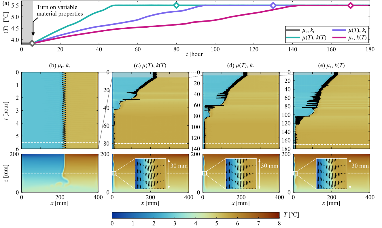
FIG. 7. Transient dynamics from constant to variable material properties in VC with T_h = 8^{\circ}\text{C} and H = 200 mm. (a) Mean temperature profiles \langle T \rangle . The shaded period corresponds to that for the constant material properties, and the variable material properties are selectively turned on afterwards. Hovmöller diagram of temperature T obtained at the middle depth z = H/2 = 100 mm (middle) and snapshot of temperature field (bottom) for different conditions: (b) \mu_r and k_r , (c) \mu(T) and k(T) , (d) \mu(T) and k_r , and (e) \mu_r and k(T) . The snapshots correspond to the symbols in (a) and the dashed lines in the Hovmöller diagram. Insets in (c), (d), and (e) showcase the close-up of the vicinity of the wall with the superposition of velocity vectors.
