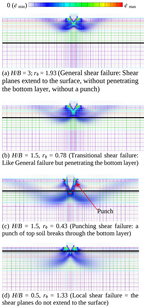
Fig. 8 Failure patterns
