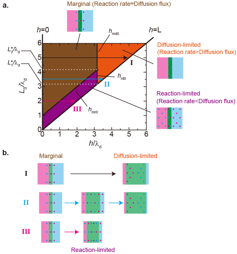
Figure 3 Regime diagram without material flow. a. Regime diagram of rate-limiting processes of mechanochemical reactions with respect to product-rich layer thickness h(t) and system size L_0 . The diagram was constructed using the expressions in Tables 2–4 with \alpha = 0.01 and \beta = 10.0 . The diffusion-limited, reaction-limited, and marginal regimes are shown in orange, purple, and brown, respectively. Without flow in the product-rich layer, the system thickness L_0 remains constant, whereas the thickness h(t) of the product-rich layer increases over time (trajectories indicated by black, cyan, and magenta arrows). The marginal/diffusion-limited, marginal/reaction-limited, and reaction-limited/diffusion-limited crossover boundaries are denoted by h_{md0} , h_{mr0} , and h_{rd0} , respectively. The sequence of crossovers experienced by the system depends on L_0 of the system with three thresholds \lambda_d , L_1^* , and L_2^* . b. Schematic illustration of the crossover sequences corresponding to the black, cyan, and magenta trajectories shown in panel a .
