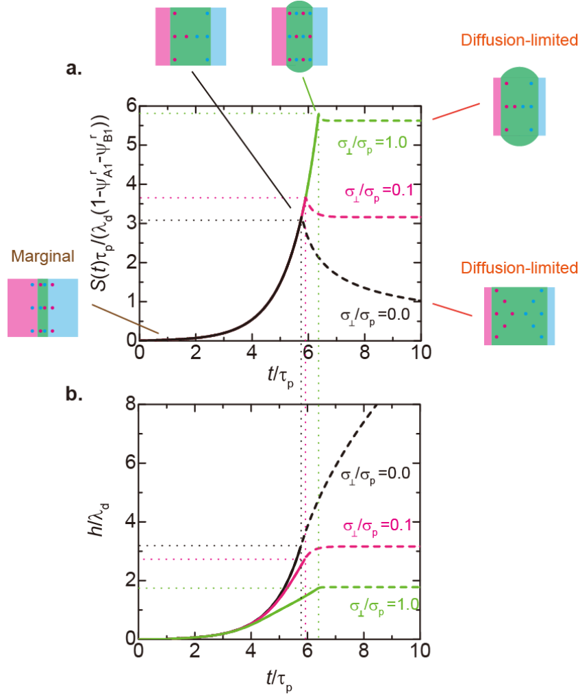
Figure 4 Reaction rate vs time. The reaction rate S(t) (rescaled by the scale S_p ) (a) and thickness h(t) (rescaled by the diffusion length \lambda_d ) of the product-rich layer (b) are
