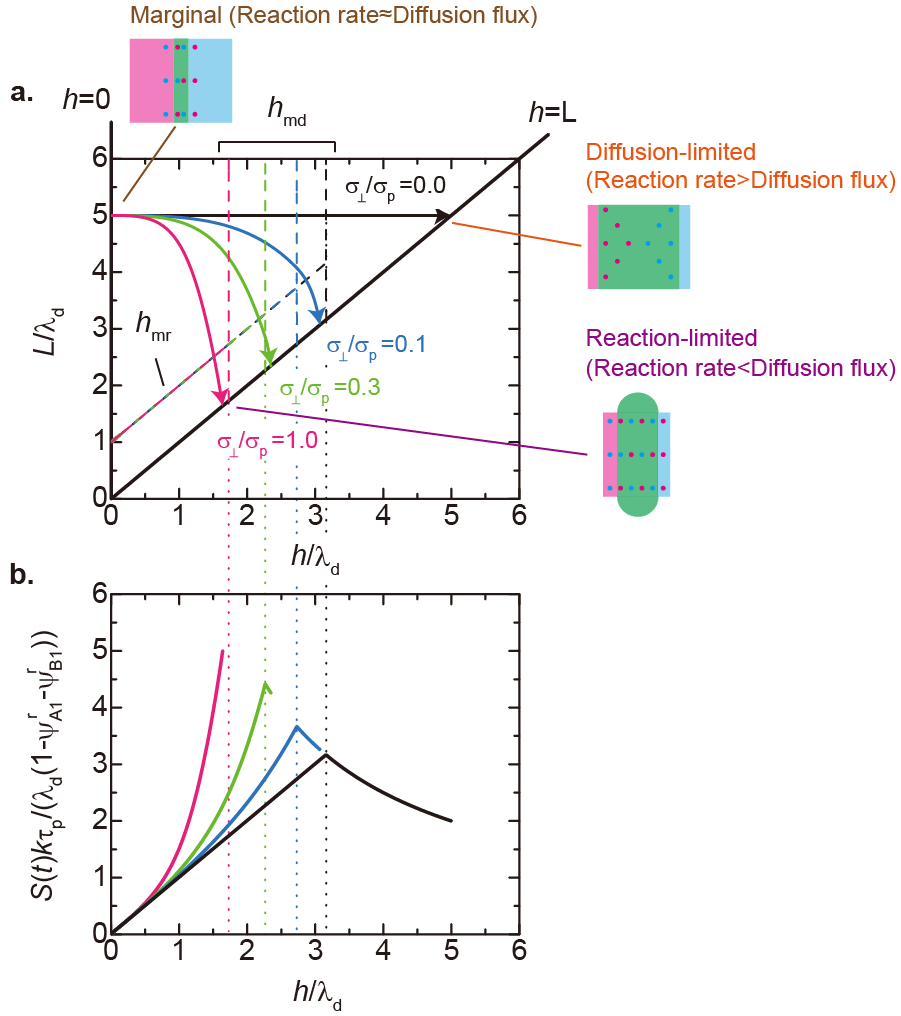
Figure 6 Reaction trajectories vs. applied mechanical stress. Trajectories (a) and reaction rates S(t) (b) of mechanochemical reactions are shown for \sigma_{\perp}/\sigma_p = 0.0 (black), 0.1 (cyan), 0.3 (light green), and 1.0 (magenta) as a function of the product-rich layer thickness h(t) and the system size L(t) . The results were obtained by numerically integrating eqs. (5) and (6) for \alpha = 0.01 , \beta = 10.0 , and L_0/\lambda_d = 5.0 . The dotted lines correspond to crossover boundaries separating marginal, diffusion-limited, and reaction-limited regimes (see also Fig. 3).
