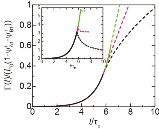
Figure 7 Conversion ratio vs. time. The conversion ratios \Gamma(t)/L_0 (rescaled by the product volume fraction 1 - \psi_{A1}^r - \psi_{B1}^r \approx 1 in the product-rich phase) are shown as a function of rescaled time t/\tau_p for \sigma_{\perp}/\sigma_p = 0.0 (black), 0.1 (magenta), 1.0 (light green) with \alpha = 0.01 , \beta = 10.0 , and L_0/\lambda_d = 10.0 . The rescaled conversion ratio \Gamma(t)/L_0 is derived by integrating the rescaled reaction rate S(t)\tau_p/(\lambda_p(1 - \psi_{A1}^r - \psi_{B1}^r)) (shown in the inset) with respect to the rescaled time t/\tau_p and then by dividing it with the rescaled system thickness L_0/\lambda_d .
