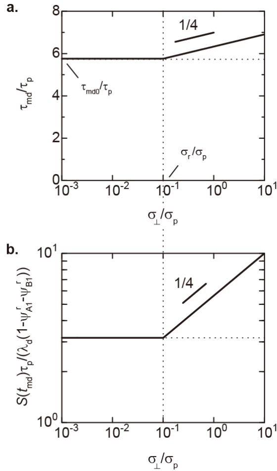
Figure 5 Marginal/diffusion-limited crossover time vs. applied mechanical stress. Characteristic time t_{\text{md}} (rescaled by the time scale \tau_p ) (a) and reaction rate S(t_{\text{md}}) (rescaled by the scale S_p ) (b) at the marginal/diffusion-limited crossover as a function of
