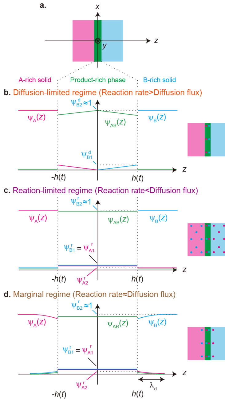
Figure 2 Volume fraction profile of reactants. a. Schematic showing the coordinate system, where the x–y plane is located at the mid-plane of the product-rich layer (green) and the z-axis is normal to the plane. The volume fractions of reactants A (magenta) and B (cyan) as well as product AB (green) are presented as functions of the position z for the diffusion-limited (b), reaction-limited (c), and marginal regimes (d).
