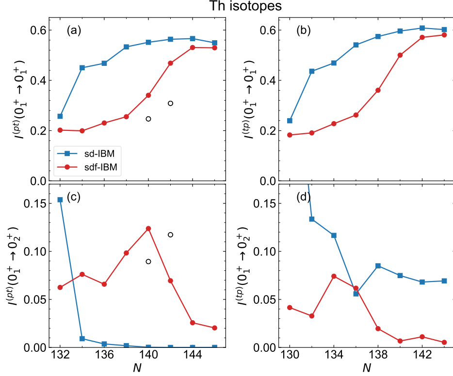
FIG. 9. Same as the caption to Fig. 8, but for the Th isotopes. Experimental data for the ^{230}\text{Th}(p,t)^{228}\text{Th} and ^{232}\text{Th}(p,t)^{230}\text{Th} , adopted from Ref. [26], are differential cross sections in \mu\text{b/sr} units measured at the laboratory angle of 7.5^\circ .
