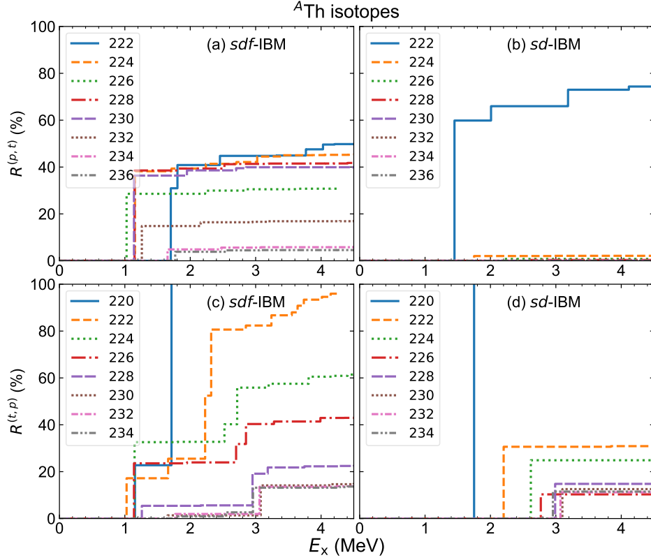
FIG. 11. Same as the caption to Fig. 10, but for the ^{A+2}\text{Th}(p,t)^A\text{Th} and ^A\text{Th}(t,p)^{A+2}\text{Th} reactions with A = 220 - 234 .
