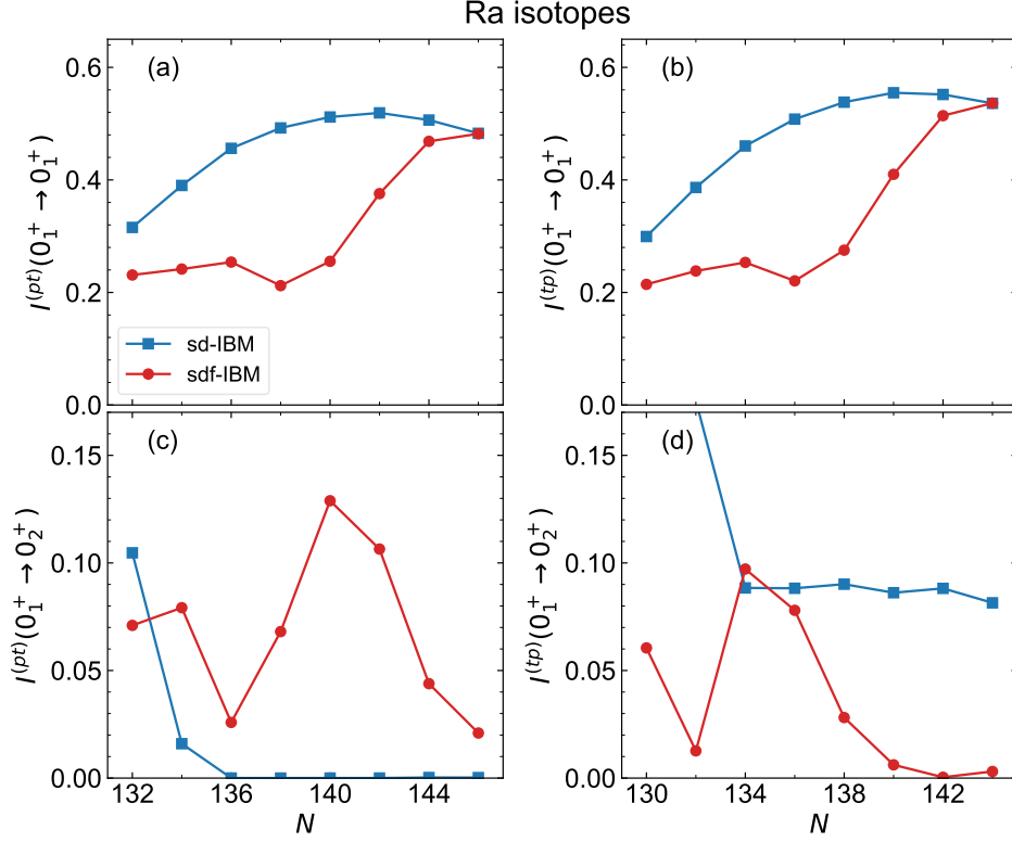
FIG. 8. (p, t) and (t, p) transfer intensities in Ra isotopes depicted as functions of N of the initial nucleus. Results obtained from the mapped sdf -IBM are compared with those from the sd -IBM.
