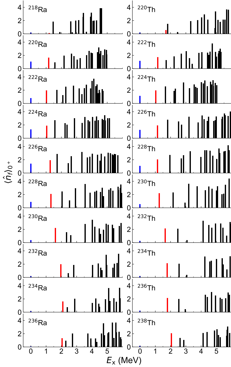
FIG. 4. Expectation values of the f -boson number operator, \langle \hat{n}_f \rangle_{0_n^+} ( n \geq 1 ), in the 0_n^+ states in Ra and Th isotopes, plotted against the corresponding energies, E_x . The \langle \hat{n}_f \rangle_{0_1^+} and \langle \hat{n}_f \rangle_{0_2^+} values are highlighted in color blue and red, respectively.
