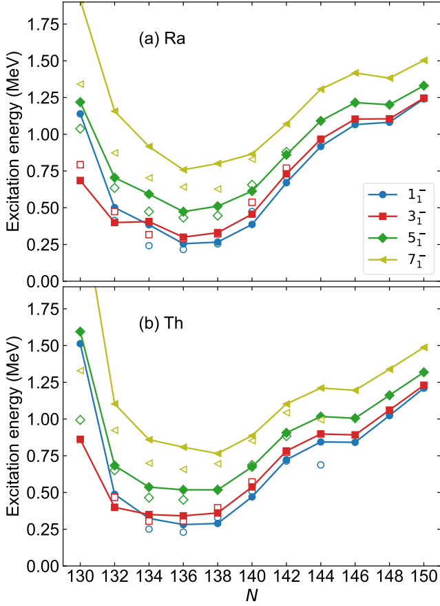
FIG. 2. Energy spectra for the odd-spin negative-parity yrast states obtained from the mapped sdf -IBM, represented by the solid symbols connected by the solid lines. Experimental data, adopted from Ref. [66], are depicted as open symbols.
