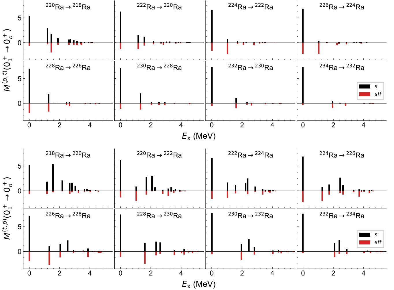
FIG. 6. Calculated matrix elements, (11)–(14) with n \geq 1 , for the ^{A+2}\text{Ra}(p,t)^A\text{Ra} (upper) and ^A\text{Ra}(t,p)^{A+2}\text{Ra} (lower) reactions with A = 218 - 232 , plotted against the excitation energies E_x in the final nucleus. In each plot, the absolute values of the s -boson contributions, |M_s^{(p,t)}(0_1^+ \rightarrow 0_n^+)| and |M_s^{(t,p)}(0_1^+ \rightarrow 0_n^+)| (denoted “ s ”), are shown, while the f -boson contributions are shown with their sign being negative, that is, -|M_{sff}^{(p,t)}(0_1^+ \rightarrow 0_n^+)| and -|M_{sff}^{(t,p)}(0_1^+ \rightarrow 0_n^+)| (denoted “ sff ”).
