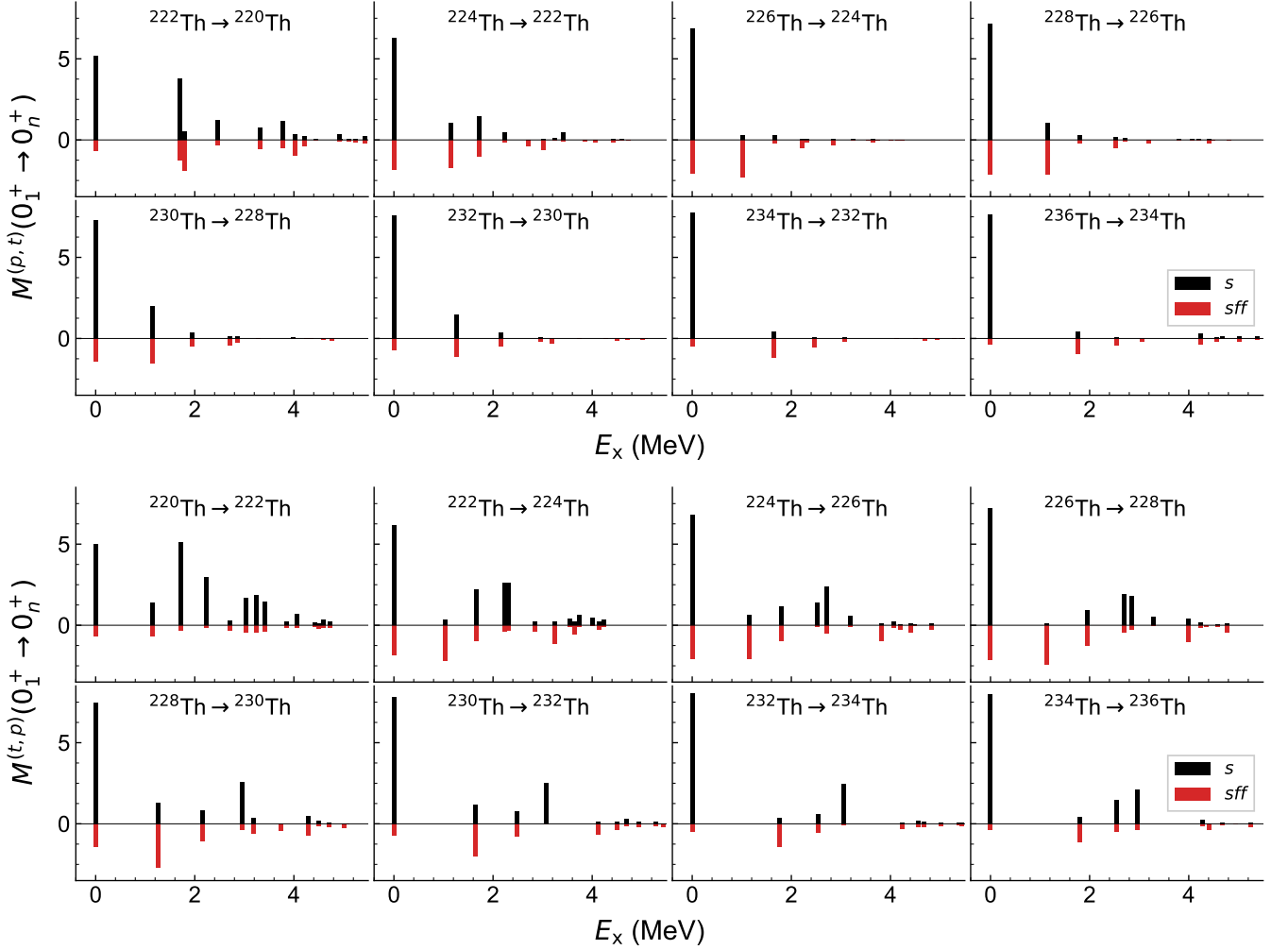
FIG. 7. Same as the caption to Fig. 6, but for the ^{A+2}\text{Th}(p,t)^A\text{Th} (upper) and ^A\text{Th}(t,p)^{A+2}\text{Th} (lower) reactions with A = 220 - 234 .
