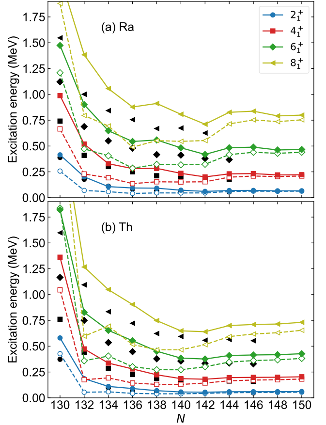
FIG. 1. Energy spectra of even-spin positive-parity yrast states in Ra and Th isotopes calculated with the mapped sd\bar{f} -IBM and sd -IBM, represented by the solid and open symbols connected by the solid and dashed lines, respectively. The experimental data are adopted from Ref. [66], and are shown as the black solid symbols.
