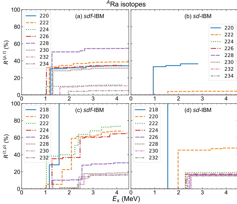
FIG. 10. Running sums, R^{(p,t)} and R^{(t,p)} , for ^{A+2}\text{Ra}(p,t)^A\text{Ra} and ^A\text{Ra}(t,p)^{A+2}\text{Ra} reactions with A = 218 - 232 , respectively. Results from the sdf -IBM [(a) and (c)] and sd -IBM [(b) and (d)] are compared.
