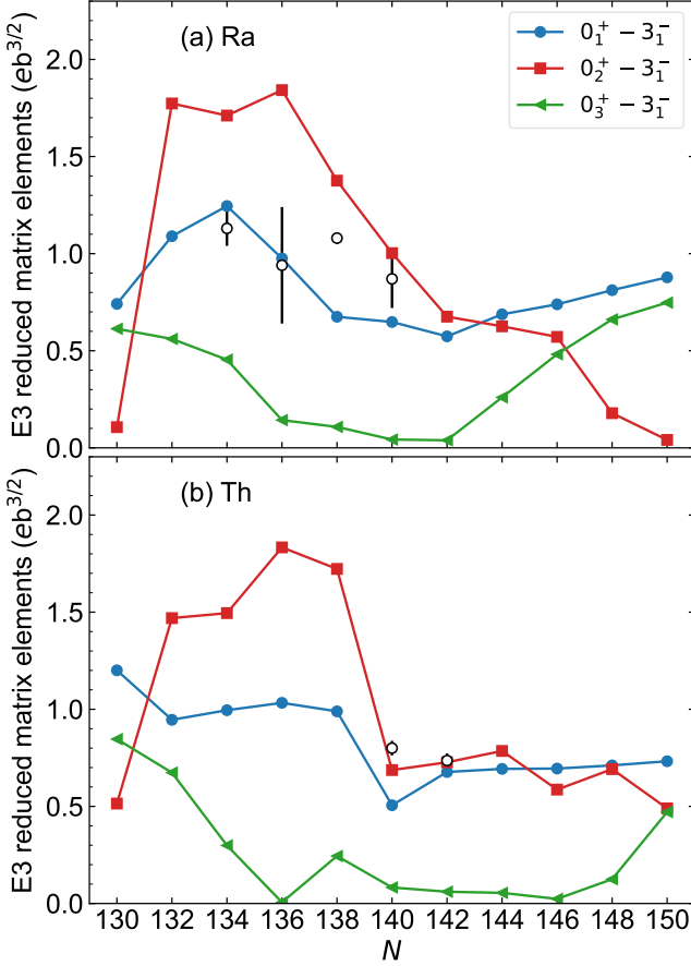
FIG. 5. Absolute values of the calculated reduced matrix elements |\langle 3_1^- || \hat{T}(E3) || 0_1^+ \rangle| , |\langle 3_1^- || \hat{T}(E3) || 0_2^+ \rangle| , and |\langle 3_1^- || \hat{T}(E3) || 0_3^+ \rangle| in eb^{3/2} units. Experimental |\langle 3_1^- || \hat{T}(E3) || 0_1^+ \rangle| values for ^{222,228}\text{Ra} [67], ^{224}\text{Ra} [7], ^{226}\text{Ra} [68], ^{230}\text{Th} [69], and ^{232}\text{Th} [70] are represented by open circles.
