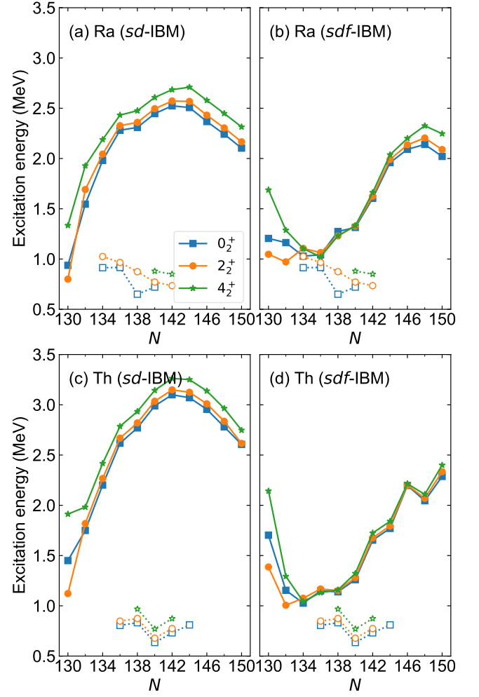
FIG. 3. Predicted excitation energies of nonyrast states, 0_2^+ , 2_2^+ , and 4_2^+ , within the sd -IBM [(a) and (c)] and sdf -IBM [(b) and (d)], represented by the solid symbols connected by the solid lines. The corresponding experimental data, adopted from Ref. [66], are depicted as open symbols connected by dotted lines.
