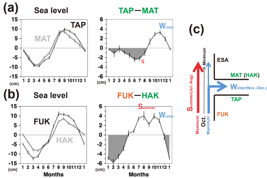
Fig. 4. The same as Fig. 3, but these figures use sea levels at (a) MAT and TAP, and (b) FUK and HAK, which are located on opposite sides of the Tsugaru Strait. The sea level difference between these two locations is considered an indicator of surface geostrophic flow passing through the strait; however, the time series for (a) and (b) exhibit different seasonal variations. (c) Schematic diagram showing that only winter-intensified disturbance can penetrate into the strait.
