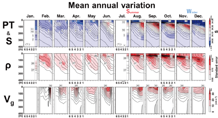
Fig. 8. Monthly mean vertical cross sections of the 15-year averaged potential temperature PT , salinity S , potential density \rho , and geostrophic current velocity V_g — calculated from the horizontal density gradient between two adjacent points, referring a depth of 400 dbar as level of no motion.
