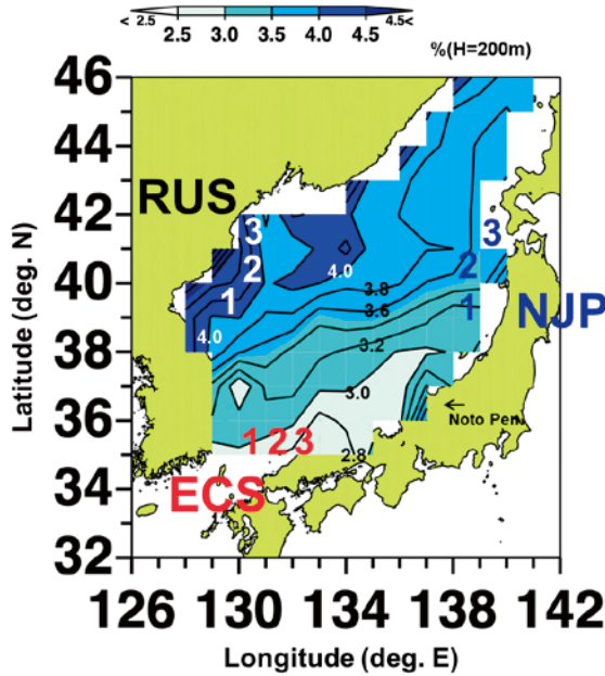
Fig. 10. Horizontal distribution of the annual average freshwater content \%(H = 200 \text{ m}) . In the Japan Sea, this content exhibits one area of minimum and two areas of maxima, referred to as ECS, RUS, and NJP, respectively. The numbers 1-3 refer to the three grids selected to illustrate seasonal variations across the three regions (ECS, NJP, and RUS).
