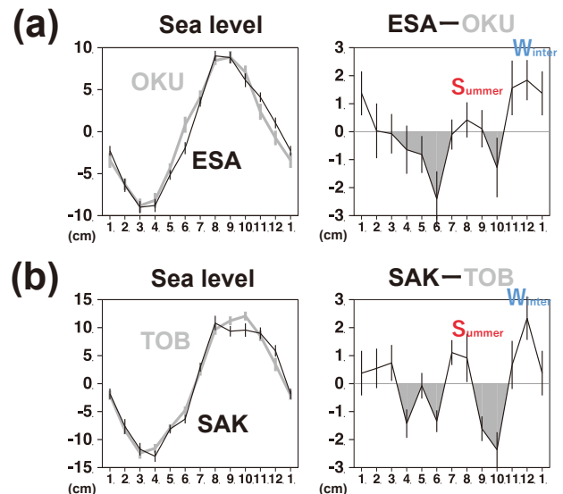
Fig. 3. The left and right panels show the mean annual variations of sea level at offshore island and its neighboring Japanese coast, and their difference used as an indicator of surface geostrophic flow. (a) refers the two stations OKU and ESA to the north of the Tsugaru Strait, and (b) TOB and SAK to the south of the strait. The vertical bars for each month represent the standard error.
