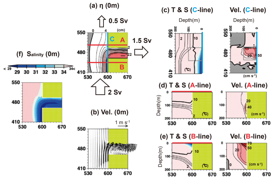
Fig. 17. The same as Fig. 16, but for horizontal and vertical distributions around the strait channel during Stage 3 on Day 70. Since freshwater inflow occurs at this stage, we have added a salinity legend and the horizontal distribution of surface salinity in (f).
