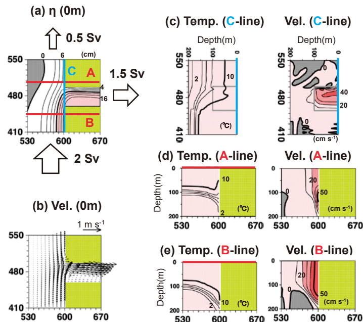
Fig. 16. The same as Fig. 14, but for horizontal and vertical distributions around the strait channel during Stage 2 on Day 40
