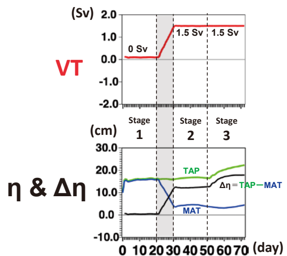
Fig. 15. The lower panel shows the time variation of the sea levels at MAT and TAP (blue and green lines) and their difference \Delta\eta = \text{TAP} - \text{MAT} (black line), and the upper panel shows that of forced volume transport VT (red line) through the strait channel.
