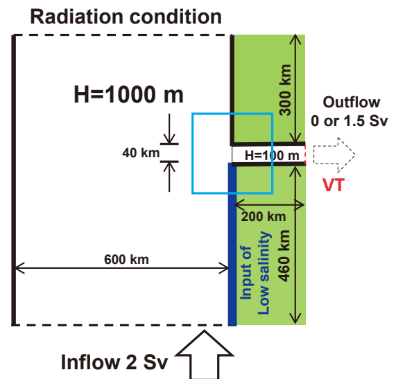
Fig. 13. Model domain consisting of a rectangular sea representing the deep Japan Sea, with a straight channel representing the shallow Tsuruga Strait connected to its eastern side.
