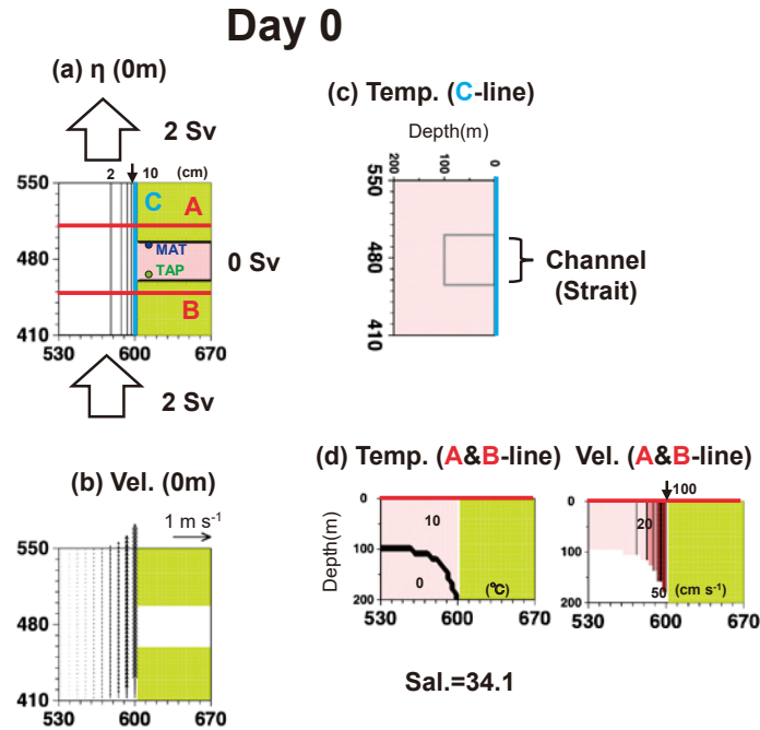
Fig. 14. Initial conditions for a summer warm-water-driven density current. Horizontal distributions of (a) sea level and (b) surface velocity vector. Vertical distributions of (c) temperature along C line, and (d) temperature and current velocity normal component along A and B lines. Model grid points corresponding to the Matsumae (MAT) and Tappi (TAP) are indicated by circles labeled with the same abbreviations in (a).
