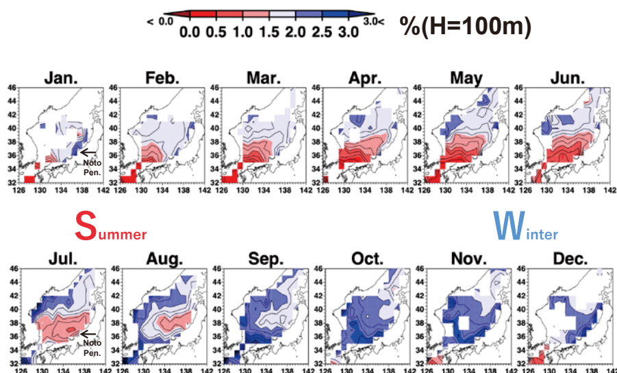
Fig. 12. Monthly change in horizontal distributions of freshwater content \%(H=100\text{ m}) of surface water in the Japan Sea.
