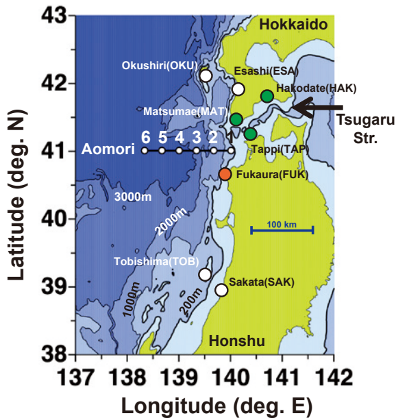
Fig. 2. Bottom topography at the western region of the Tsugaru Strait. Location of the 8 tide-gauge stations and hydrographic stations 1-6 along the Aomori line, used in this study.
