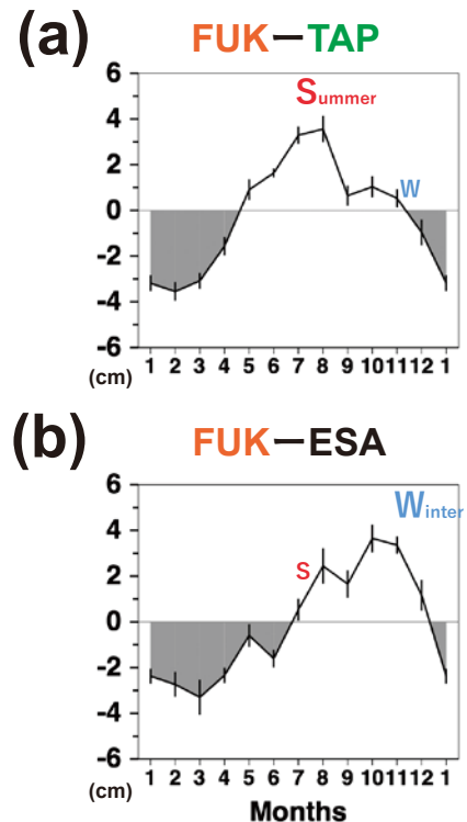
Fig. 5. The same sea level difference as Figs. 3 and 4, but for (a) FUK-TAP and (b) FUK-ESA.
