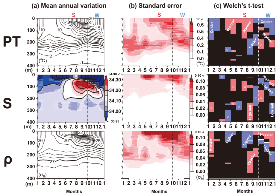
Fig. 6. (a) shows the depth-time diagrams of mean annual variations of potential temperature, salinity, and (b) is their standard errors. (c) shows the Welch's t -test, which accounts for the standard errors of these values. In this test, areas where the value for the given month differs statistically significantly from the previous month's value (using a 95% significance level) are displayed in red, while areas showing a decrease are displayed in blue; areas where no significant difference is observed are displayed in black.
