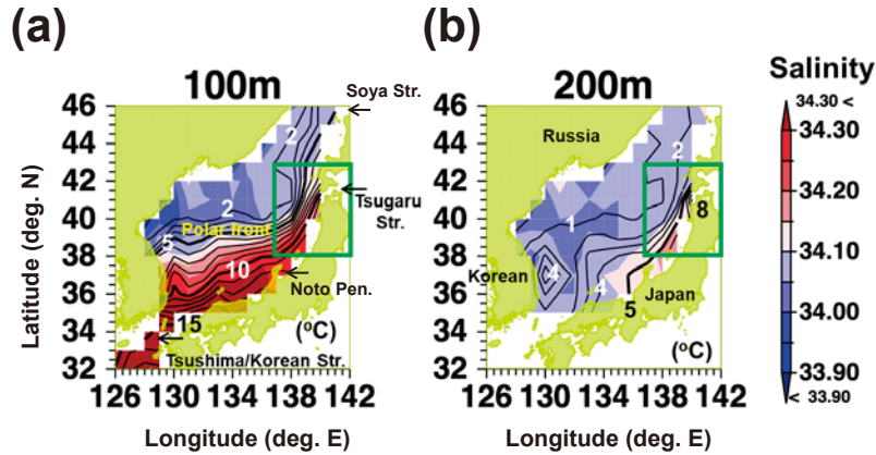
Fig. 1. Horizontal distributions of annual mean salinity and water temperature at (a) a depth of 100 m and (b) a depth of 200 m, based on climatological averages from 1906 to 2003. The green box indicates the western region of the Tsugaru Strait, which is the study area shown in Fig. 2.
