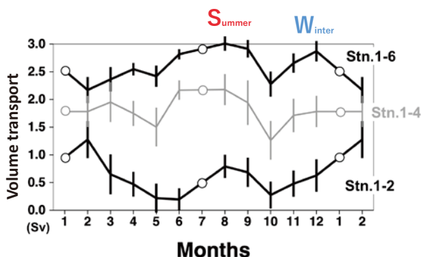
Fig. 9. Monthly time series in cumulative volume transport for three categories, i.e., the cumulative totals for Stations 1-2 are shown as a black line, those for Stations 1-4 as a gray line, and those for Stations 1-6 as a black line. Since the transports cannot be calculated for January and July, the open circles for those two months indicate linear interpolation, and the vertical bars represent the standard error for each month.
