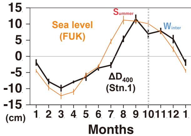
Fig. 7. The solid black line indicates the monthly variation in dynamic height \Delta D_{400} , while the solid orange line indicates that of sea level at FUK; the vertical bars on both time series represent their respective standard errors.
