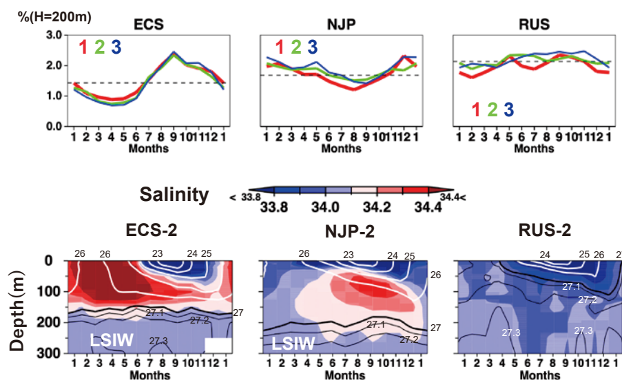
Fig. 11. The upper panels show the monthly changes in the percentage of freshwater content \%(H = 200 \text{ m}) in three grid cells selected from each sea area (ECS, NJP, and RUS), and lower panels show the depth (0-300 m)-time diagrams of salinity, using grid number 2 as a representative example. The contour lines superimposed on the salinity isopleths indicate density.
