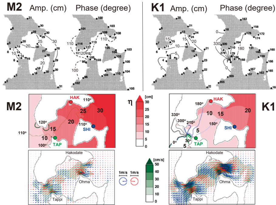
Fig. 11. Amplitude and phase charts of M2 and K1 tides estimated from tidal harmonic constants based on the coastal tide-gauge stations (Matsuura and Isoda, 2020) are shown at upper panels. Middle and lower panels are the model results for the spatial distributions of tidal harmonic constants of sea level and current. The amplitude and phase of sea level are shown by red shading and contour lines, respectively. Tidal current is represented by the current ellipses; clockwise is blue line, anti-clockwise is red line, and the amplitude of long axis is shown by green shading. S2 and O1 constituent charts (not shown) are almost the same patterns of M2 and K1 constituents, respectively.
