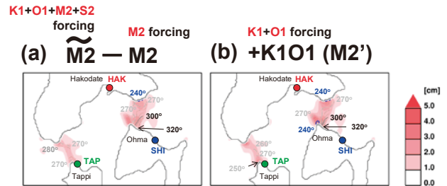
Fig. 13. Symbol \widetilde{M2} implies M2 tide obtained from K1 + O1 + M2 + S2 forcing model, M2 is the true M2 tide obtained from M2-only forcing model, and the compound tide M2' is given by diurnal K1 + O1 forcing model. Spatial distributions of (a) amplitude and phase calculated from \widetilde{M2} - M2 and (b) those of +K1O1 ( M2' ).
