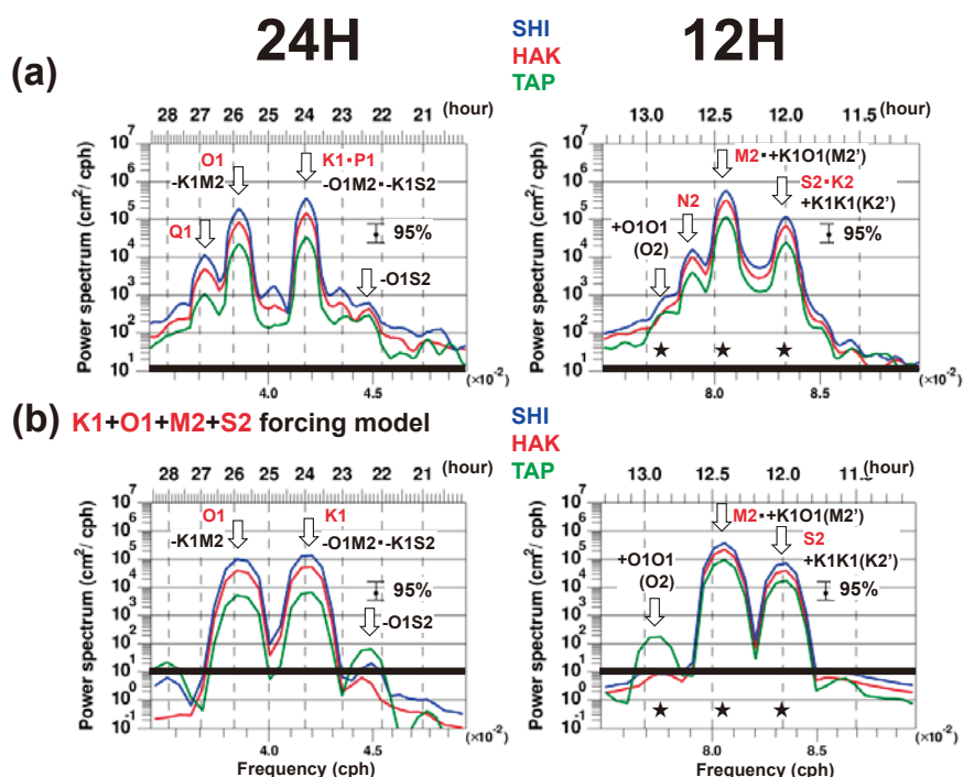
Fig. 6. Enlarged views of the power spectrum focusing on the vicinities of the 24H and 12H periods. (a) are the spectrums of the observed sea level at three tidal stations, and (b) are those of the modeled sea level at three grid points near the coastal tidal stations. Red, blue, and green solid lines denote the spectrum of Hakodate, Shimokita, and Tappi, respectively.
