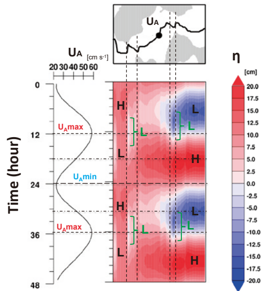
Fig. 15. Thick solid line in the upper panel indicates a flow-axis of calculated passage-flow through the strait. Lower panel show the space-time diagram of sea level variations along its flow-axis during 48 hours. Symbols H and L are sea level high and low, respectively. Left-hand side panel is time series of eastward current variation during the same 48 hours at the selected grid point of U_A , which located is indicated by a dotted point at the upper panel.
