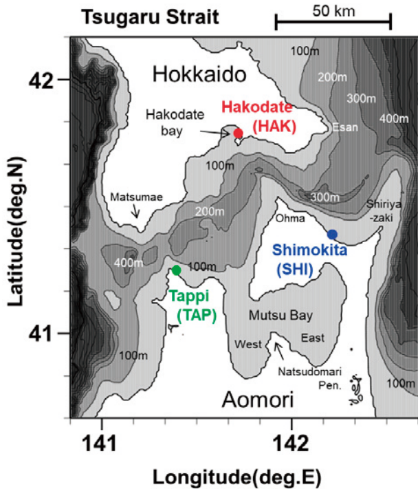
Fig. 4. Bathymetry around the Tsugaru Strait. Red, blue, and green circles denote the coastal tidal stations of Hakodate, Shimokita, and Tappi, respectively.
