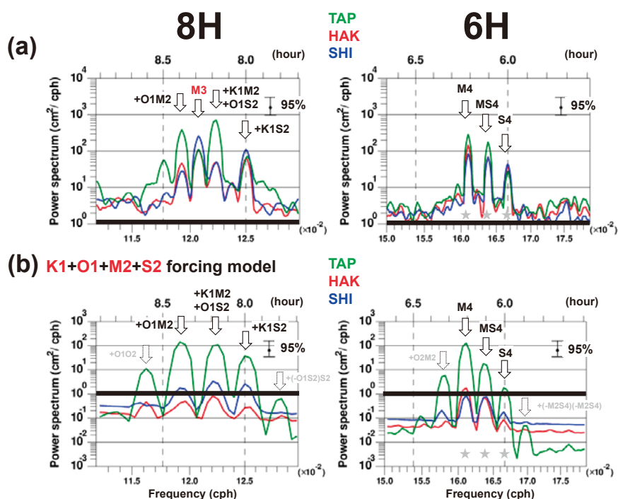
Fig. 7. Same as Fig. 6, but for the 8H and 6H periodical ranges.
