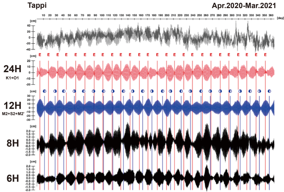
Fig. 8. Upper panel shows the time series of observed sea level at Tappi from April 2020 to March 2021. Lower four panels are 24H, 12H, 8H, and 6H band passed time series calculated by the HAB method, respectively. The vertical red and blue solid lines denote the dates of diurnal and semi-diurnal neap tides, respectively.
