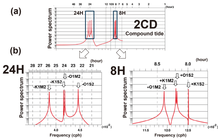
Fig. 3. (a) Power spectrum for identifying the periodicity of compound tides, comprising the time series of 2CD shown in Fig. 2. (b) Enlarged views of the power spectrum focusing on the vicinities of the 24H and 8H periods.
