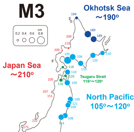
Fig. A1. Tidal harmonic constants of M3 tide at the tide-gauge stations around the northern Japan. The amplitude and phase are represented by a radius of circle and numerical, respectively, and plotted at each station.
