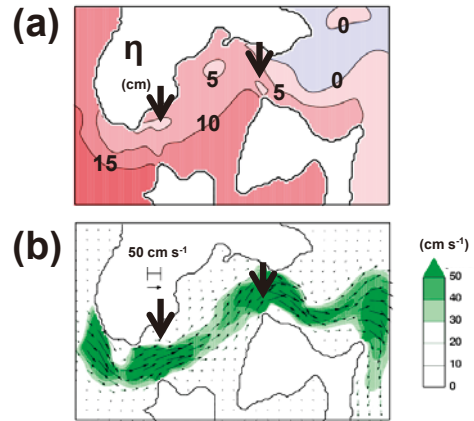
Fig. 14. Experiment for only K1 tidal forcing. Spatial distributions of (a) sea level \eta and (b) current vectors averaged over 55 days.
