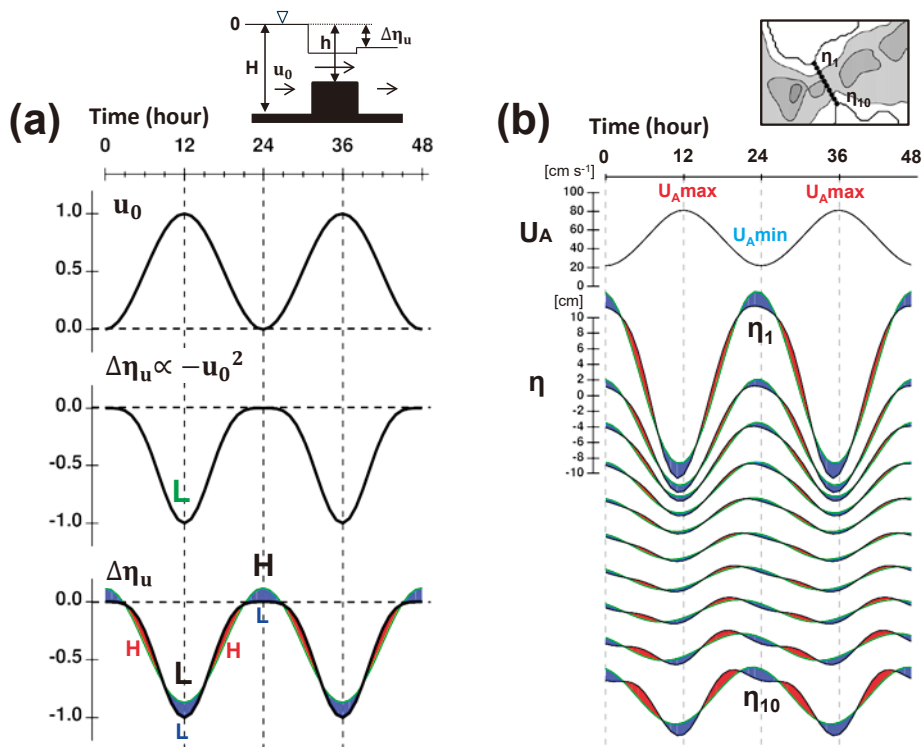
Fig. 16. Upper panel in (a) shows one-dimensional channel model for the step sill topography (Iino et al. (2009)). (a) Time series of passage flow u_0 , net sea level difference \Delta\eta_u , and anomaly from the sinusoidal wave of K1 tide, assuming u_a = u_c = 0.5 . Upper panel in (b) shows bottom topography in the western part of the strait and selected grid points on the sill. (b) is the diagram similar to (a), but the model results of U_A and sea levels from \eta_1 to \eta_{10} .
