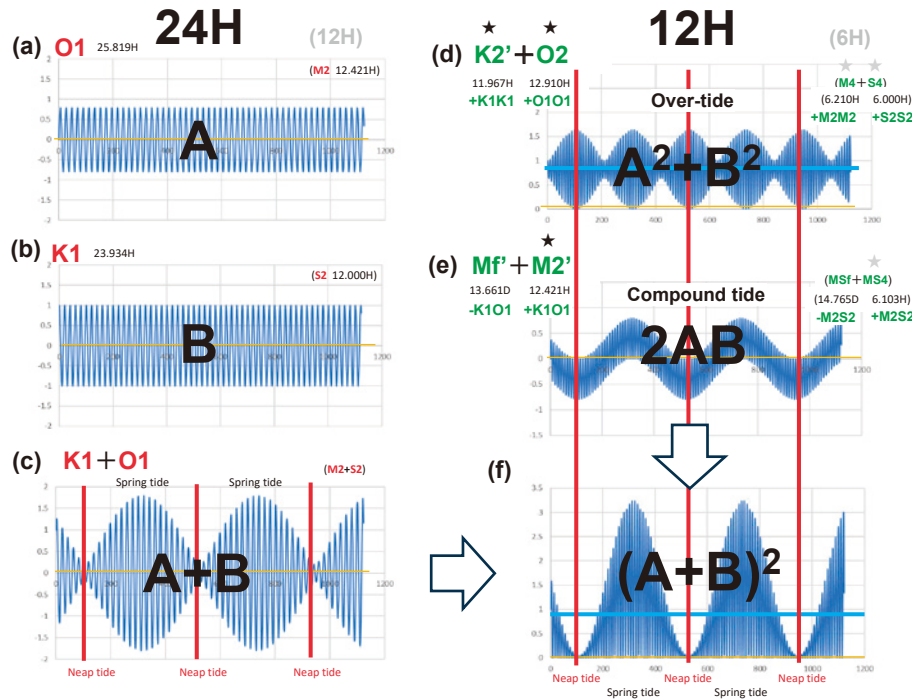
Fig. 1. Mathematical explanation of shallow-water tides using the example of diurnal tides. Time series of (a) O1 and (b) K1 tides expressed as a cosine curve. (c) K1 + O1 time-varying with diurnal spring/neap tides (period of 13.661D). The vertical red solid lines denote neap tides in which amplitude of K1 + O1 is the minimum. (d) Summation of “over-tides” generating from K1 and O1 tides ( K2' + O2 ). (e) Summation of “compound tides” generating from K1 and O1 tides ( Mf' + M2' ). (f) Summation of over-tides and compound tides ( K2' + O2 + Mf' + M2' ), which corresponds to K1 + O1 squared. In the semi-diurnal tides, (a) corresponds to M2, (b) to S2 and (c) to M2 + S2, (d) to M4 + S4, (e) to MSf + MS4, (f) to (M2 + S2) 2 .
