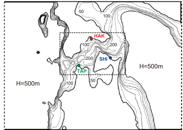
Fig. 9. Model bathymetry around the Tsugaru Strait. The northern and southern boundaries (thick black line) are artificially closed, and the western and eastern boundaries (dashed line) are opened. Water depths of regions deeper than 500 m are set to be constant 500 m. Model results only show the square area indicated by the dashed line box.
