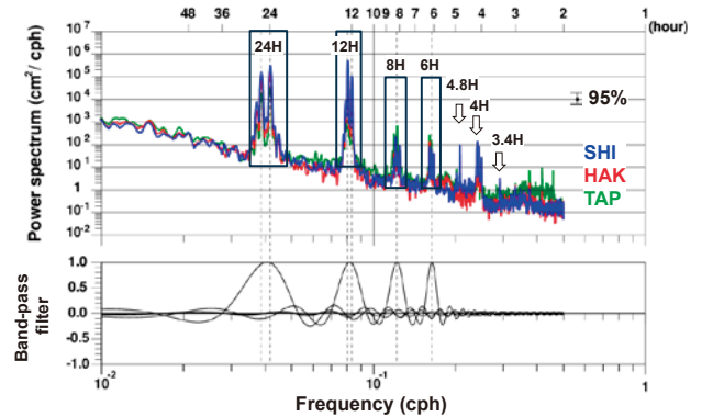
Fig. 5. (Upper panel) Power spectrum of the observed sea levels at three tidal stations. Red, blue, and green solid lines denote the spectrum of Hakodate, Shimokita, and Tappi, respectively. (Lower panel) Band-pass filter of the HAB methods to extract the periodic variations with wide frequency bands of 24H, 12H, 8H, and 6H periods.
