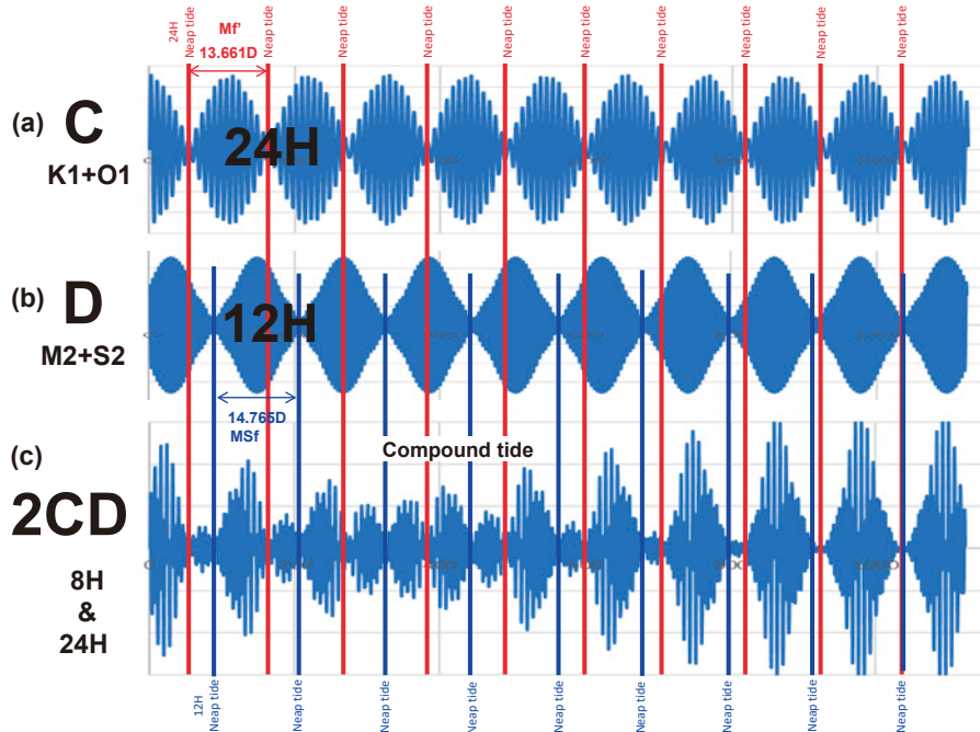
Fig. 2. Time series of the diurnal tides K1 + O1 ; C (upper panel), the semi-diurnal tides M2 + S2 ; D (middle panel), and their compound tides 2CD (lower panel). The vertical red and blue solid lines denote the dates of diurnal and semi-diurnal neap tides, respectively.
