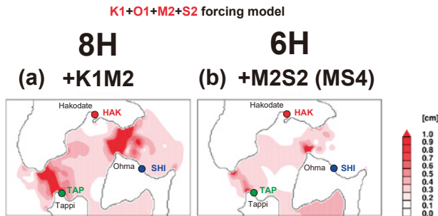
Fig. 12. Spatial distributions of tidal amplitude of (a) +K1M2 and (b) +M2S2 (MS4) as representatives of 8H and 6H periodical ranges.
