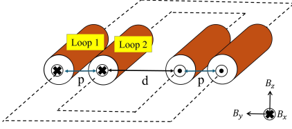
Fig. 1. Four-conductor validation model. Each conductor has radius 1.0 mm and length L = 1000 mm. The center-to-center distance between the two conductors on each side is fixed at p = 2.03 mm, whereas the center-to-center distance d between the two inner conductors is varied.
