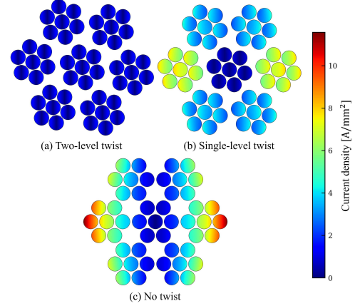
Fig. 5. Reconstructed current-density magnitude at 100 kHz under the 1-mT peak external field with zero applied voltage and zero net terminal current.
