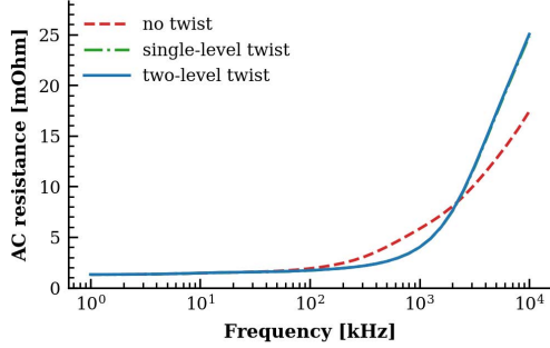
Fig. 3. AC resistance under 1-V excitation without an external magnetic field.
