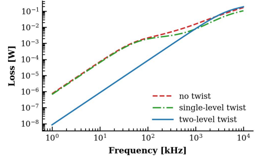
Fig. 4. Loss under a uniform 1-mT peak external field, zero applied voltage, and zero net terminal current.
