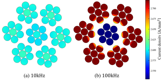
Fig. 2. Reconstructed current-density distributions of the two-level twisted lw1 model under common-terminal voltage excitation without an external magnetic field. The results are normalized to a total current of 1 A.
