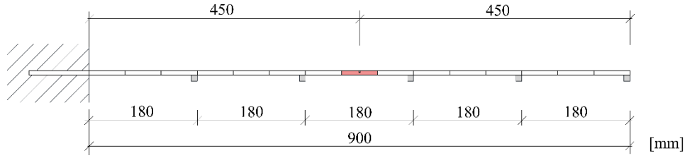
Figure 7. Scheme of cantilever beam with marked cut middle section and accelerometers.
