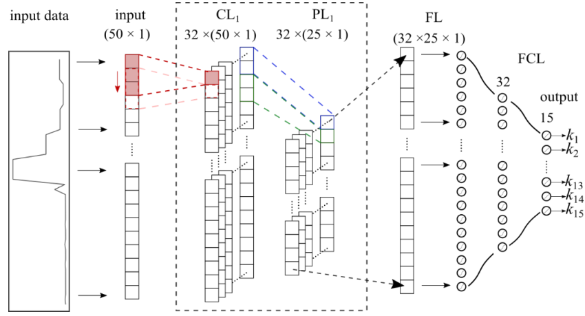
Figure 8. Scheme of architecture of CNN for wooden cantilever beam.
