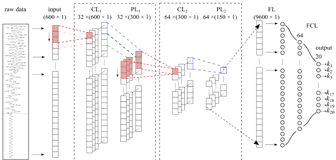
Figure 4. Scheme of architecture of CNN for riveted truss bridge.
