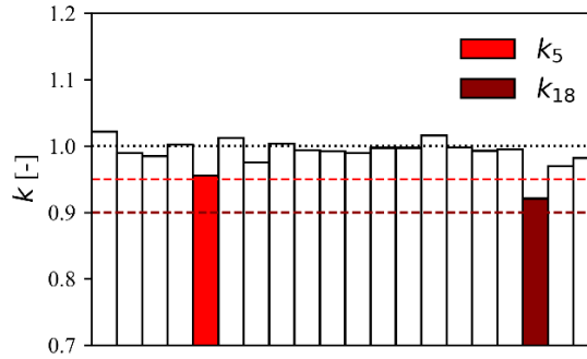
Figure 5. Stiffness scheme of diagonal members with marked damage.
