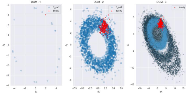
Figure 1: Reconstructed inputs via KNN for the three DGMs
