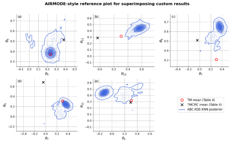
Figure 4. Selected bivariate marginals of the AIRMODE posterior distribution. Posterior samples and KDE contours from the proposed method are compared with the reference, Grashorn et al. (2024)
