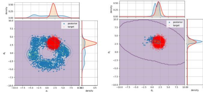
Figure 2 Posterior (blue) vs target density (red) for the DGM-2 (right) and DGM-3 (left).
