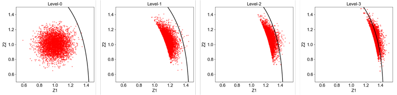
Figure 2. Schematic illustration of the evolution of SS-generated samples in a two-dimensional uncertainty space.
