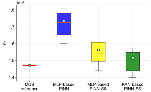
Figure 8. Failure probability estimates for the thin square plate from 10 independent MCS using different surrogate methods.
