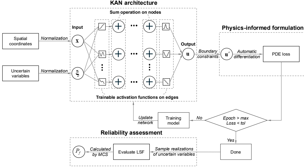
Figure 1. Workflow of the proposed KAN-based PINN framework for structural reliability analysis.
