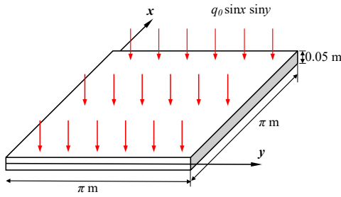
Figure 7. Schematic of a thin square plate with a sinusoidally distributed load.
