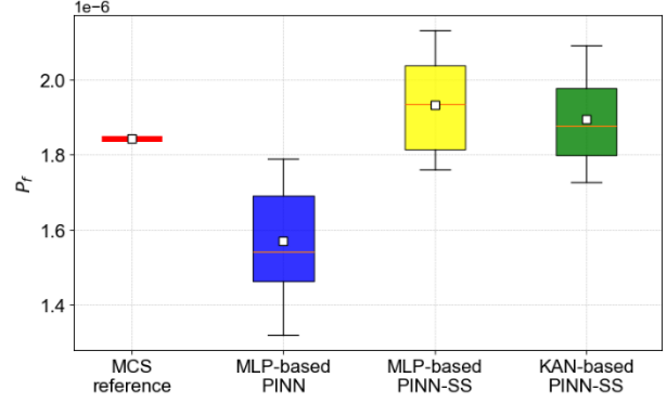
Figure 4. Failure probability estimates for the straight bar from 10 independent MCS using different surrogate methods.
