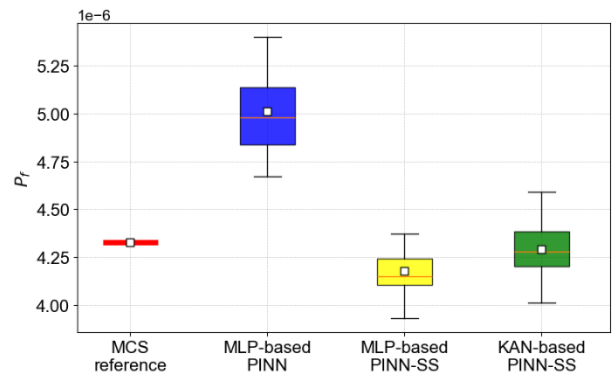
Figure 6. Failure probability estimates for the cantilever beam from 10 independent MCS using different surrogate methods.
