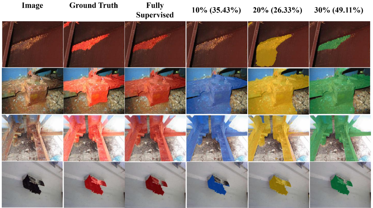
Figure 3. Detected Results for Different Supervised Fractions.
