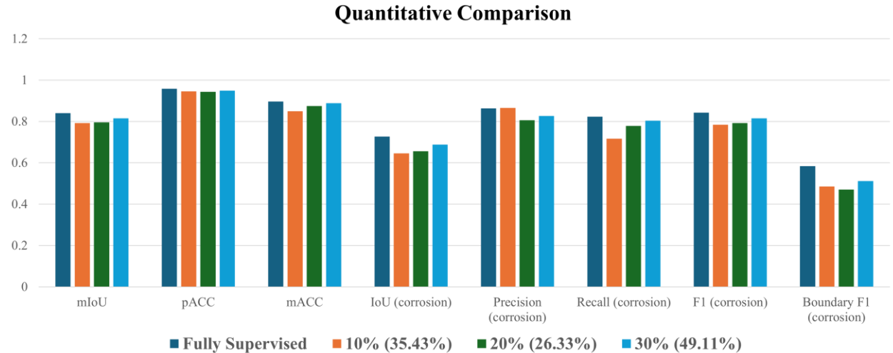
Figure 2. Quantitative performance comparison of the proposed ASSL framework and fully supervised baseline.
