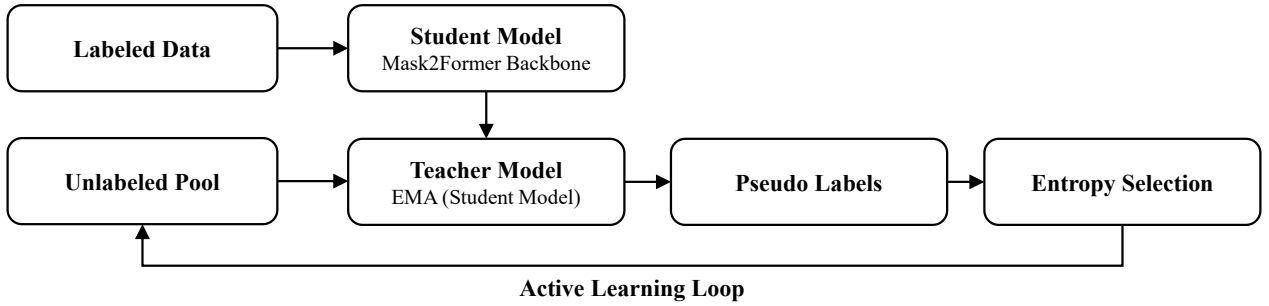
Figure 1. Proposed Active Semi-Supervised Learning (ASSL) Framework.
