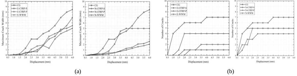
Figure 2. (a) Crack width of each specimen; (b) Number of cracks of each specimen.
