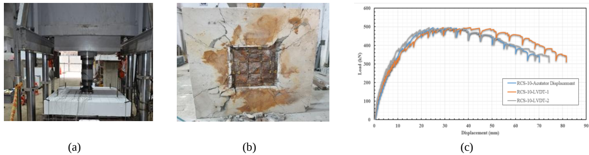
Figure 5. (a) RCS-10 specimen during monotonic loading; (b) Crack pattern at the final stage; (c) load-displacement diagram.
