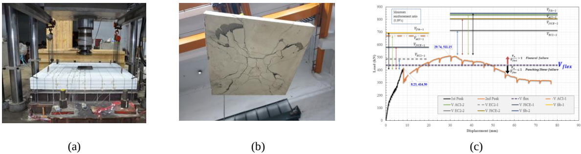
Figure 4. (a) RCS-0 specimen during monotonic loading; (b) Crack pattern at the final stage; (c) load-displacement diagram.
