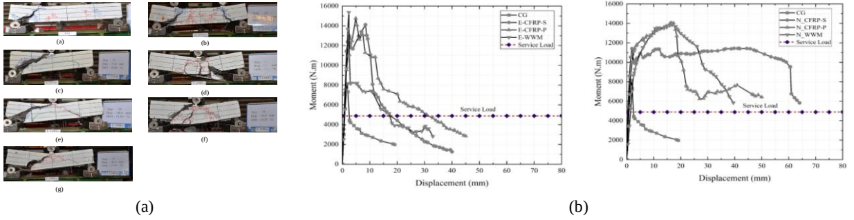
Figure 3. (a) Crack patterns at the final stage of each specimen; (b) Moment-displacement curve of repaired specimens for lightweight epoxy mortar and non-shrinkage cement mortar.
