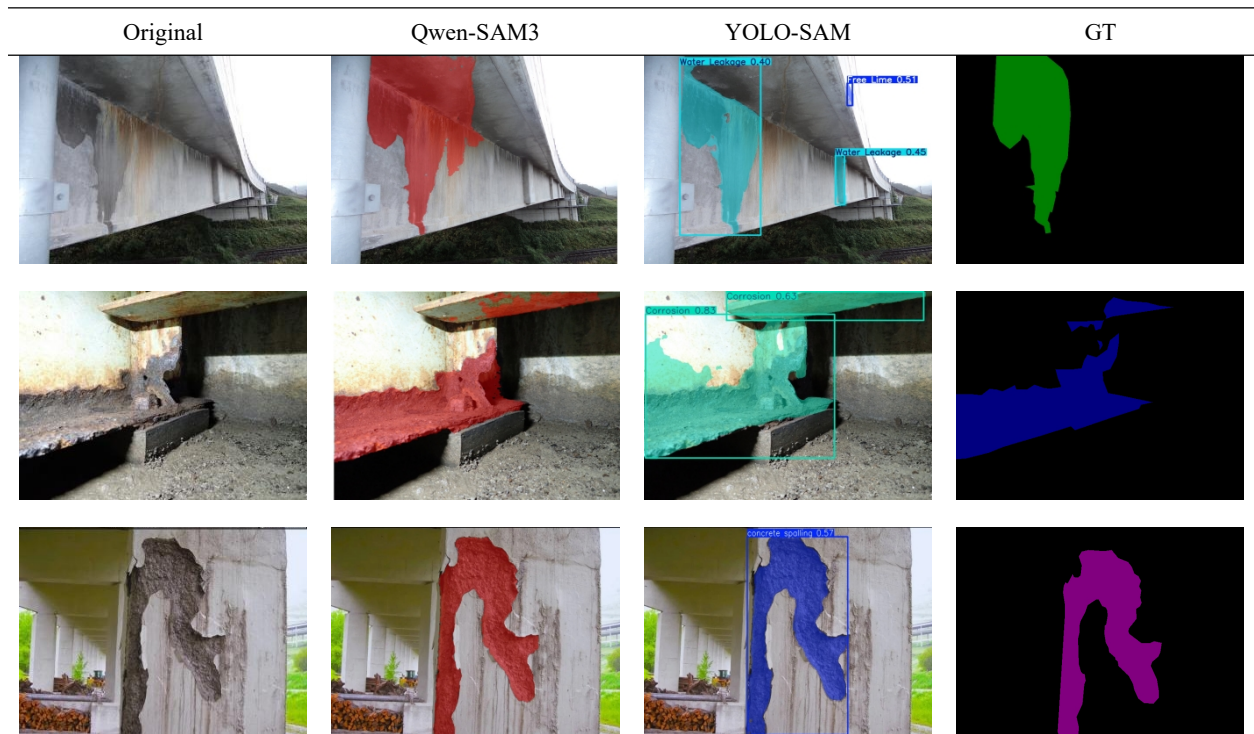
Figure 5. Comparison of different models
