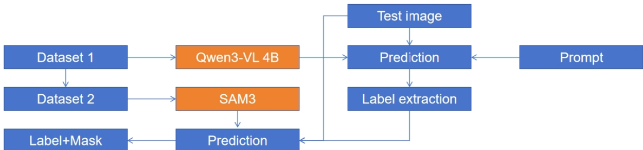
Figure 1. Overview of pipeline
