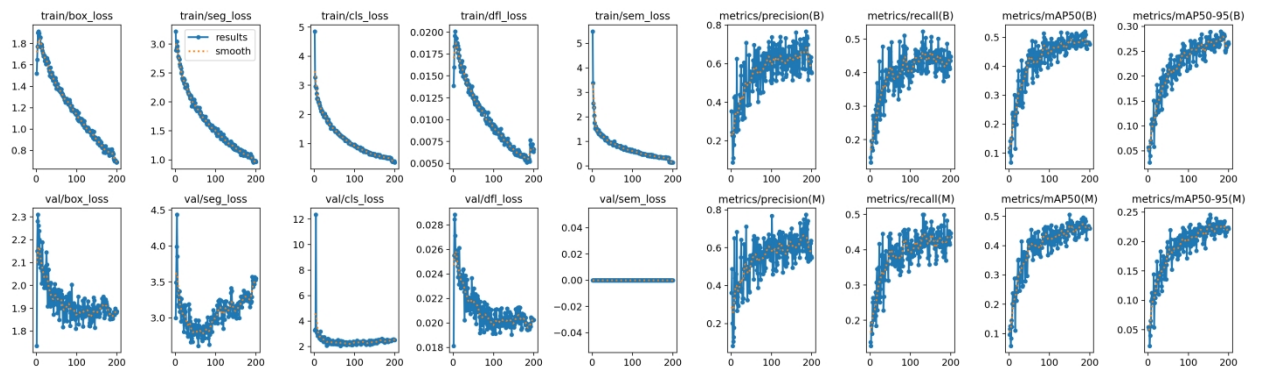
Figure 3. Result of YOLO-SAM hybrid model
