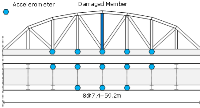
Figure 1. Schematic outline of the target bridge
