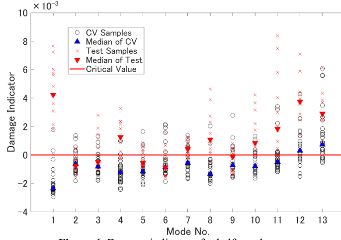
Figure 6. Damage indicators for half-cut damage
