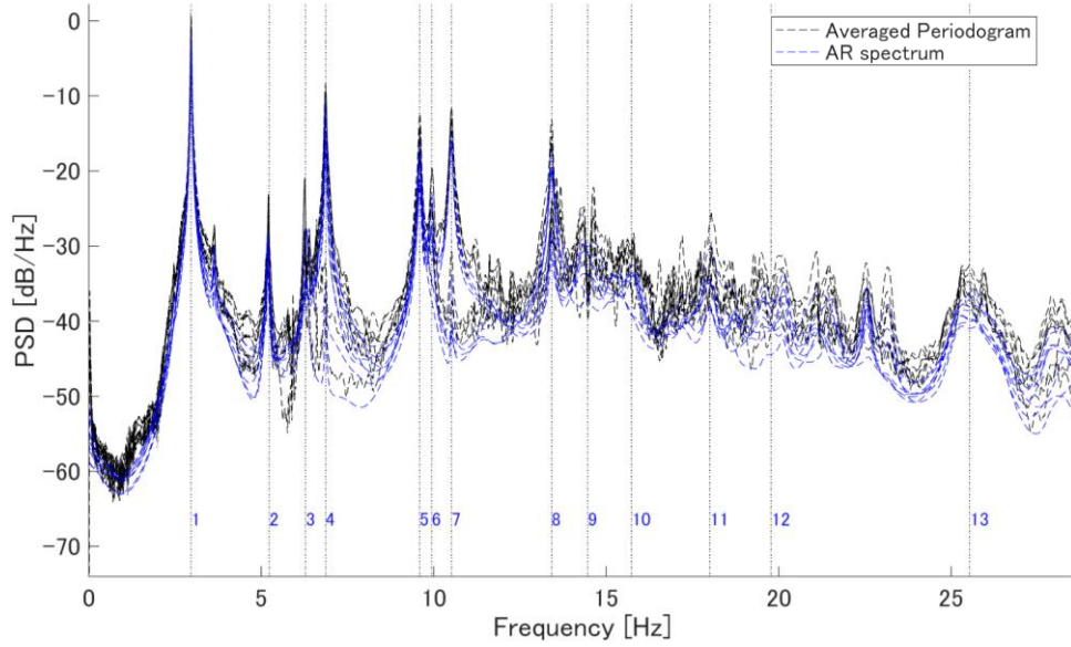
Figure 4. The trained spectrum and extracted modal frequencies
