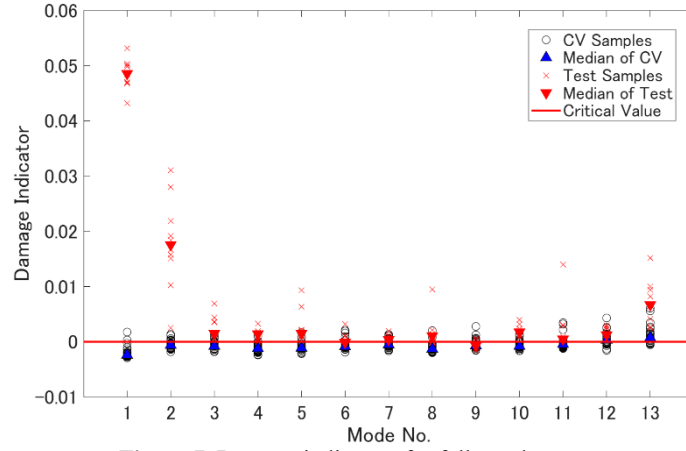
Figure 7. Damage indicators for full-cut damage
