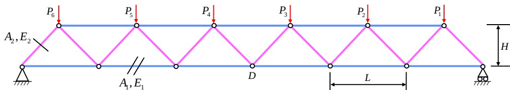
Figure 2. The 23-bar truss structure
