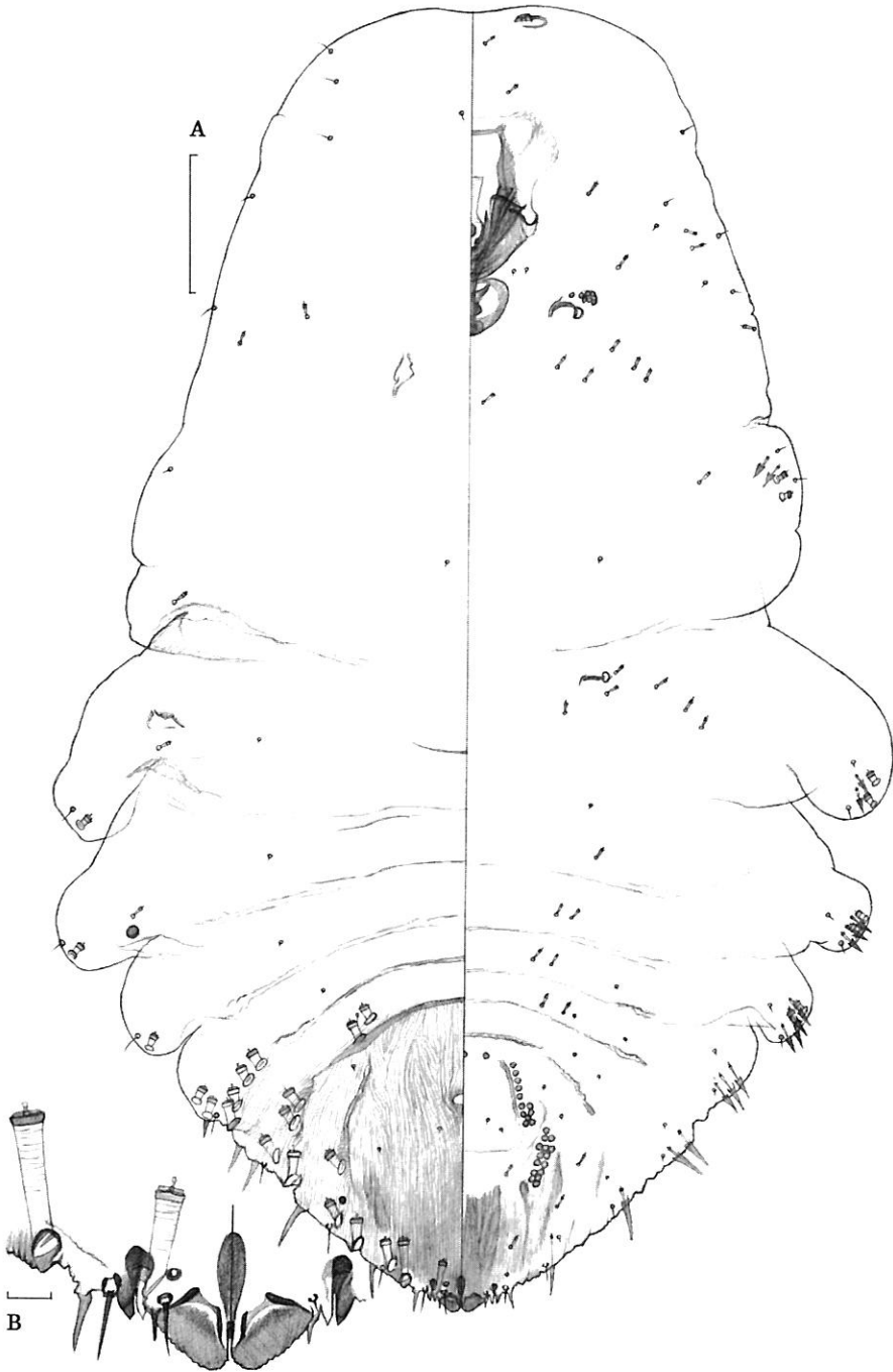
Fig. 9. Chionandaspis 91Kc-H, adult female. B, apical margin of pygidium, dorsal view. Scale bars: A, 100µm; B, 10µm.
