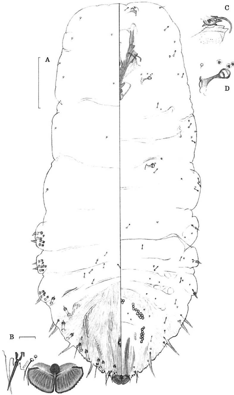
Fig. 10. Larutaspis lithocarpi , adult female. B, median and second trullae, dorsal view; C, antenna and derm pocket; D, anterior spiracle. Scale bars: A, 100µm, B, 10µm (C and D magnified at the same rate as B).
