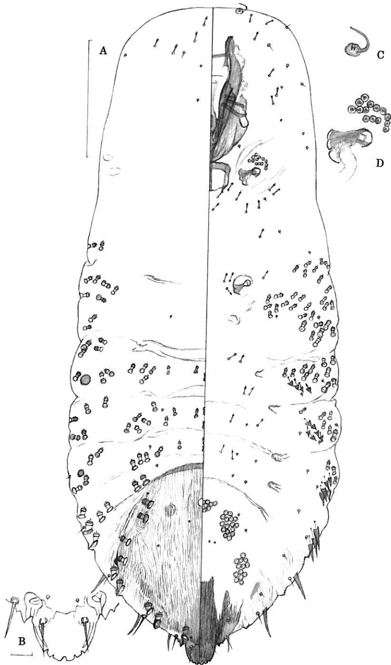
Fig. 7. Kuchingaspis hopeae , adult female. B, median trullae, dorsal view; C, antenna; D, anterior spiracle. Scale bars: A, 100µm; B, 10µm (C and D magnified at the same rate as B).
