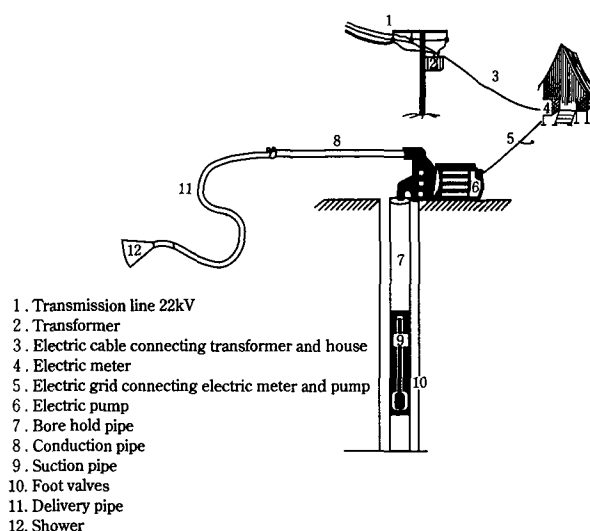
Figure 3 Tube well, pump and electric system
