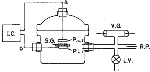
Fig. 1. The glow discharge apparatus.
