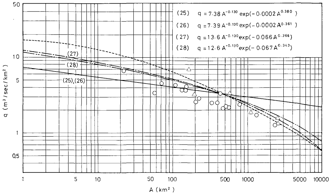
Fig. 3. Record flood peaks and curves of specific flood discharge in Hokkaido. (the upper basin of Sorachi River)
