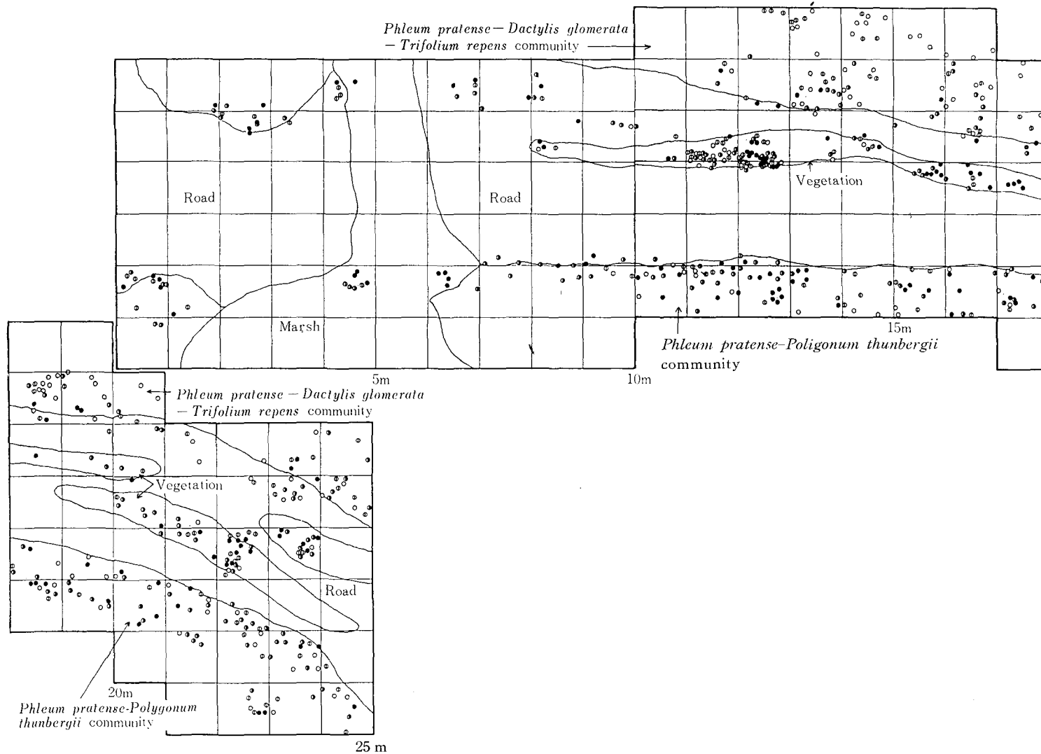
Fig. 5. Distributions of the timothy plants measured their plant type index in Site-D (6×25 m) in April 1982.
