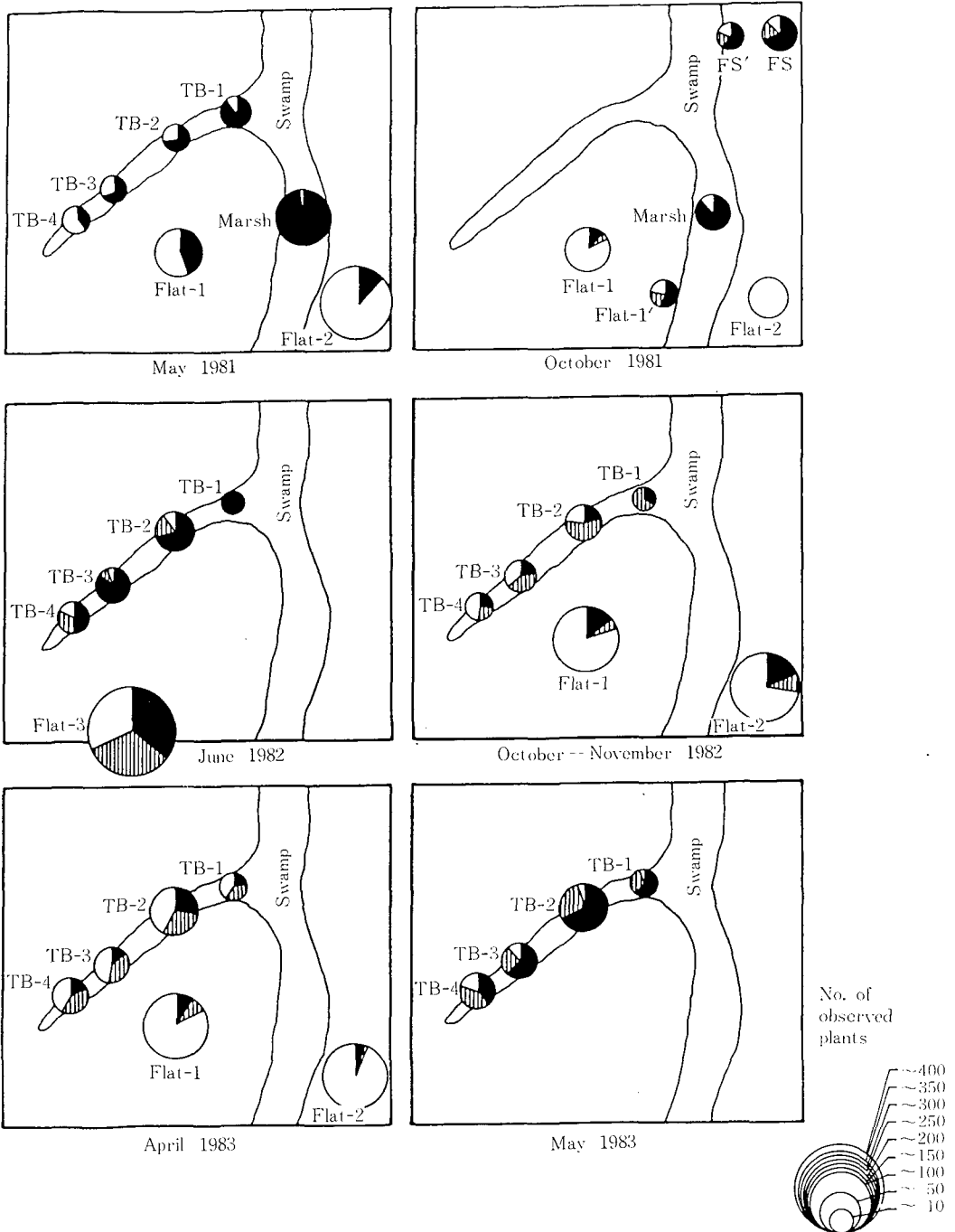
Fig. 1. Variations of plant type in several quadrats within Site-B (40×45 m) on the six dates from May 1981 to May 1983. Circle sizes are proportionate to the number of observed plants.
