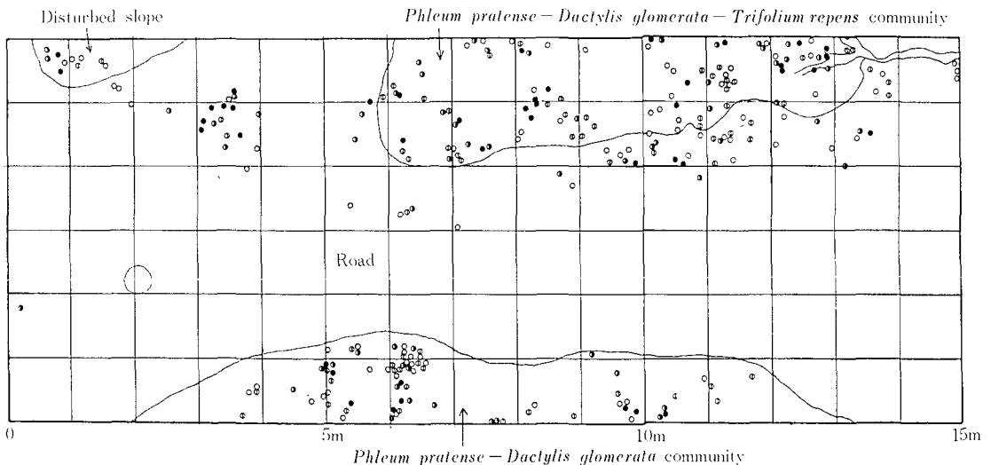
Fig. 4. Distributions of the timothy plants measured their plant type index in Site-C (6×15 m) in April 1982.
