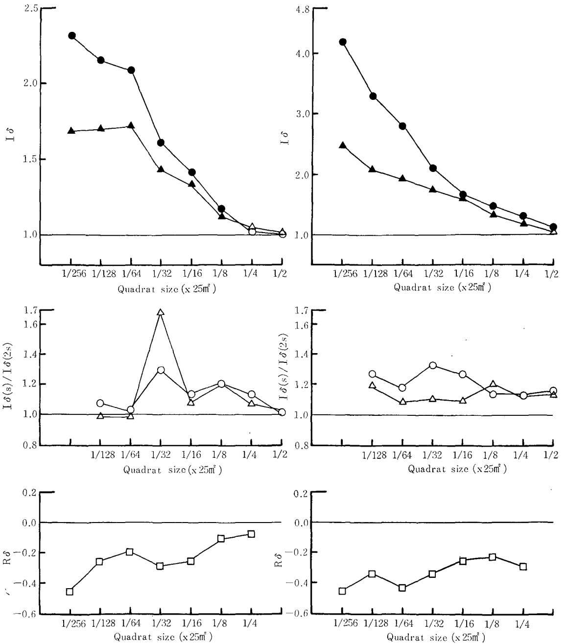
Fig. 3. I\delta -values (Upper) and I\delta(s)/I\delta(2s) -values (Middle) of the prostrate type (—○—) and the erect type (—△—) of timothy, and R\delta -values between both types (—□—, Lower) plotted against quadrat size in Flat-3 A (Left figures) and Flat-3 B (Right figures).
