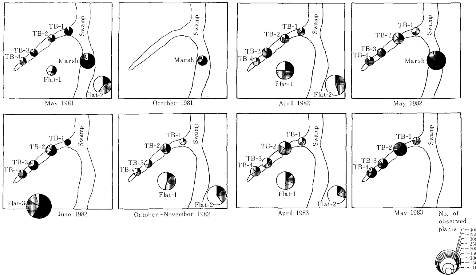
Fig. 2. Variations of plant type index in several quadrats within Site-B (40x45 m) on the eight dates from May 1981 to May 1983. Circle sizes are proportionate to the number of observed plants.
