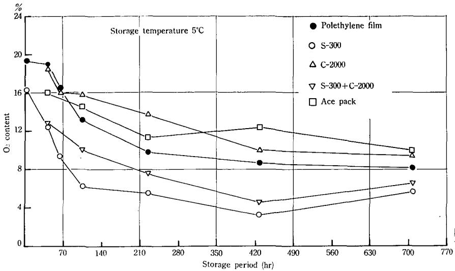
Fig. 2. Changes of O 2 content during storage (film package).
