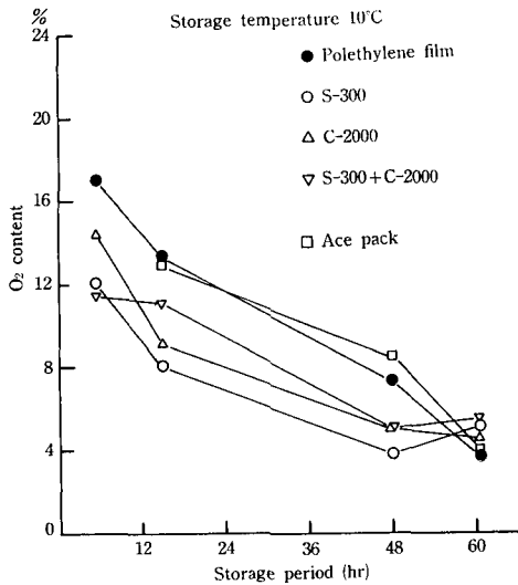
Fig. 3. Changes of O 2 content during storage (film package).
