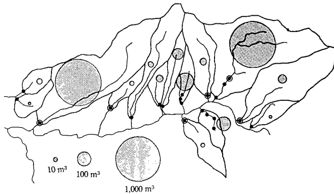
Fig. 6. Sediment conditions of each debris barriers.
