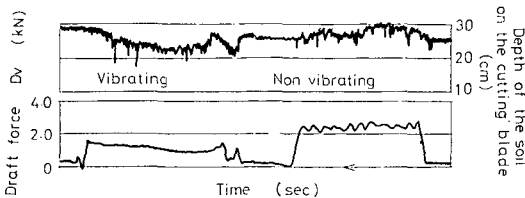
Fig. 7. Measurement of the depth of the soil on the cutting blade by a supersonic wave displacement sensor.
