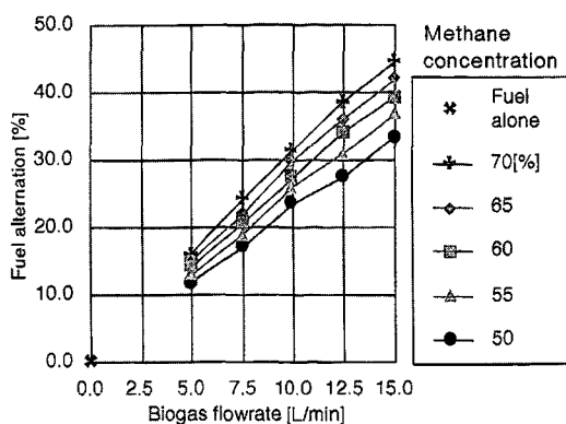
図3.2 軽油代替率の変化 Fig. 3.2 Change of diesel fuel alternation ratio
