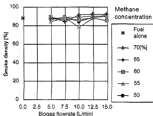
図3.4 煙濃度の変化 Fig. 3.4 Change of smoke density
