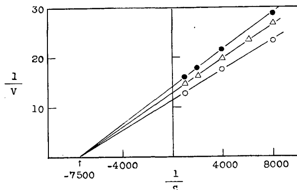
Fig. 6. Normal serum enzyme: Varying concentration of substrate and different levels of \text{Mg}^{++} , 0.025 M Veronal-HCl buffer at pH 9.7.
