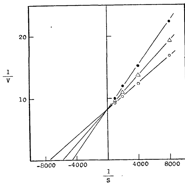
Fig. 7. THF serum enzyme: Varying concentration of substrate and different levels of \text{Mg}^{++} , 0.025 M Veronal-HCl buffer at pH 9.7.
