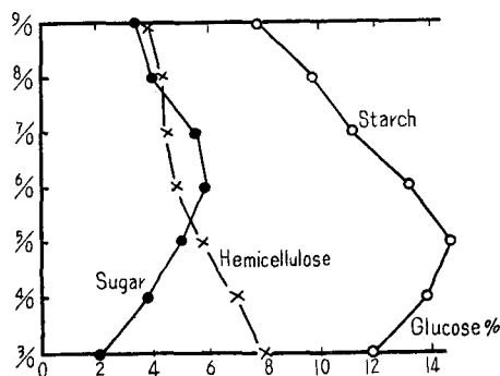
Fig. 27. Content of carbohydrates of various leaves on main stem on July 5.
