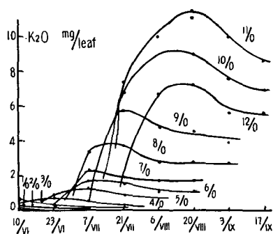
Fig. 12. Amount of potassium in each leaf at successive stages of growth.
