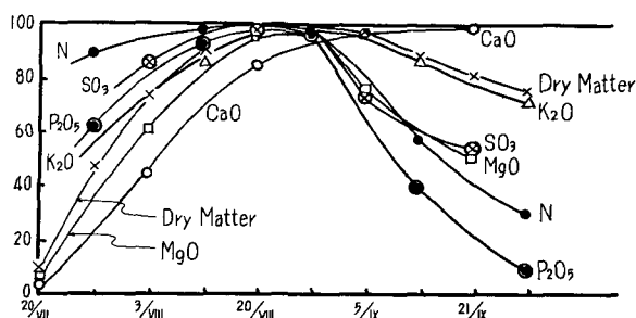
Fig. 26. Accumulation processes of elements in 11/0.
