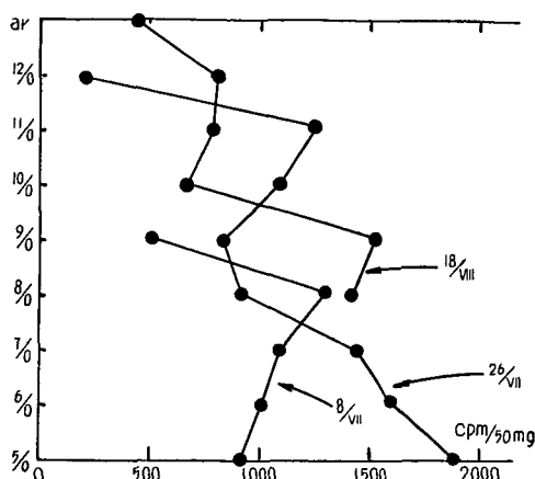
Fig. 40. Distribution of \text{Ca}^{45} absorbed from roots.
