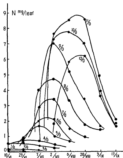
Fig. 6. Amount of nitrogen in each leaf at successive stages of growth.
