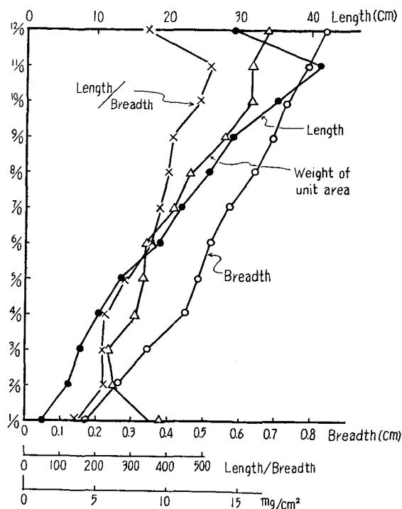
Fig. 28. Morphological characteristics of leaf-blade.
