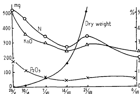
Fig. 46. Growth process of 4-tiller.
