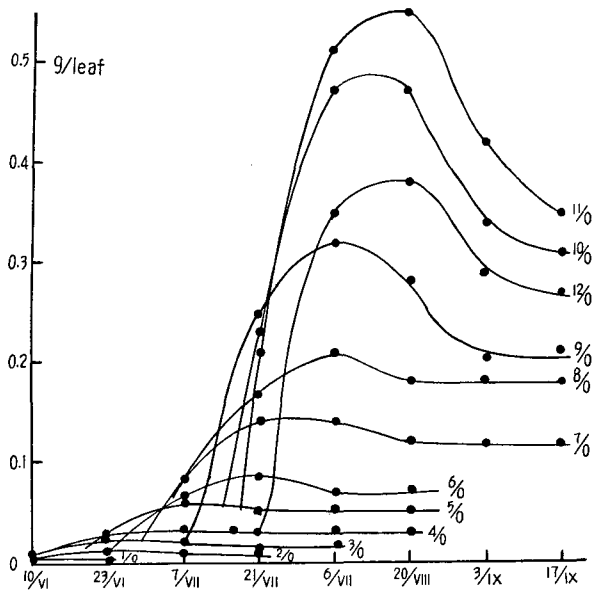
Fig. 3. Dry weight of leaves on main stem.
