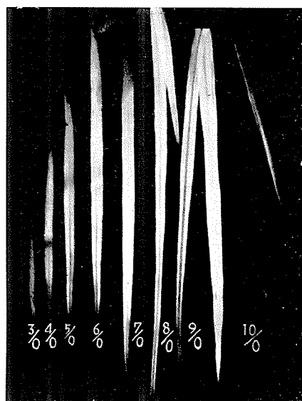
Fig. 37. Radio-autograph which shows photosynthetic activity of leaves on main stem on July 20.
