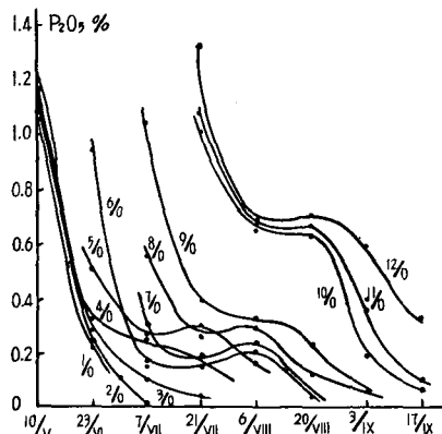
Fig. 7. Phosphorus content of each leaf on main stem at successive stages of growth.
