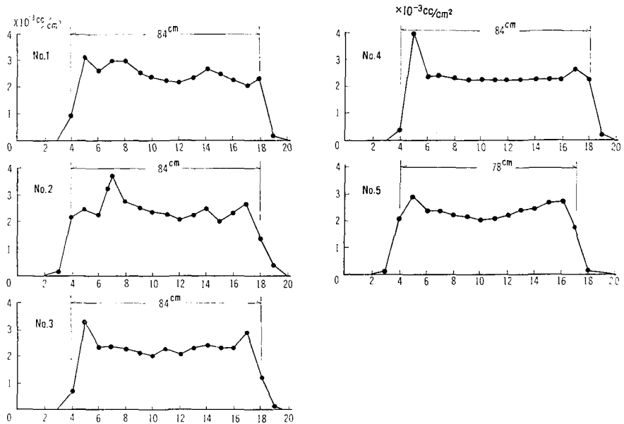
Fig. 5. The relation between discharge of nozzles and forward speed at 4 \text{ kg/cm}^2 spray pressure (Tee Jet 8003 E)
