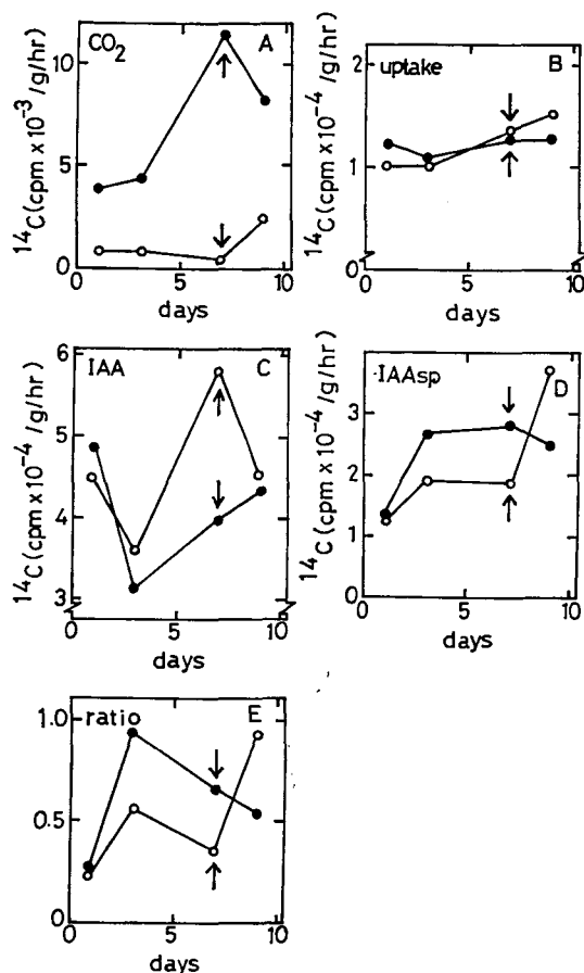
Fig. 7. Time course experiment of ^{14}\text{C} -IAA metabolism of tissue discs of potato tuber, control (—○—) and ethylene treatment (—●—), A=liberated ^{14}\text{C} - \text{CO}_2 , B=uptake of ^{14}\text{C} -IAA into the tissues, C= ^{14}\text{C} -IAA in the ethanol extracts, D= ^{14}\text{C} -IAAsp in the ethanol extracts and E=ratio of ^{14}\text{C} -IAAsp to ^{14}\text{C} -IAA.
