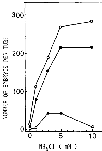
Fig. 2. Changes in number of embryos as a function of \text{NH}_4\text{Cl} level. Medium contained \text{KNO}_3 at 40 mM ( \circ — \circ ), 20 mM ( \bullet — \bullet ), or 10 mM ( \ominus — \ominus ). Determination was carried out as the same manner as Fig. 1.
