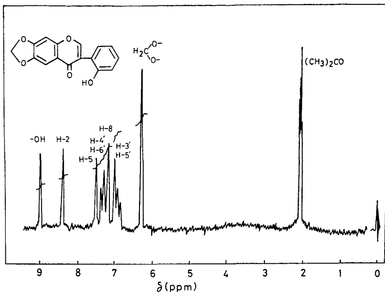
Fig. 1. NMR Spectrum of Compound I (Acetone- d_6 ).
