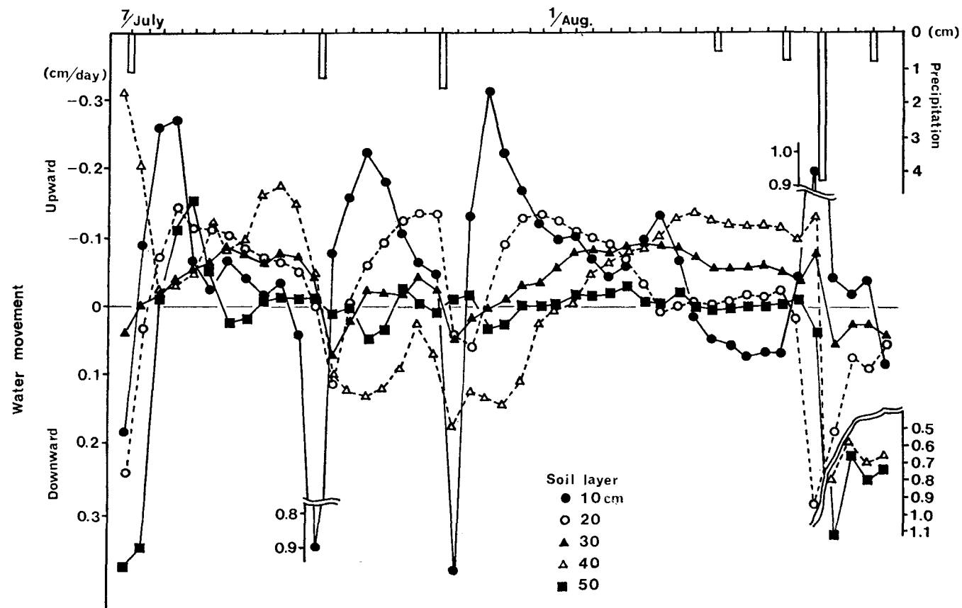
Fig. 14. Successive changes in vertical water movement (bare plot).
