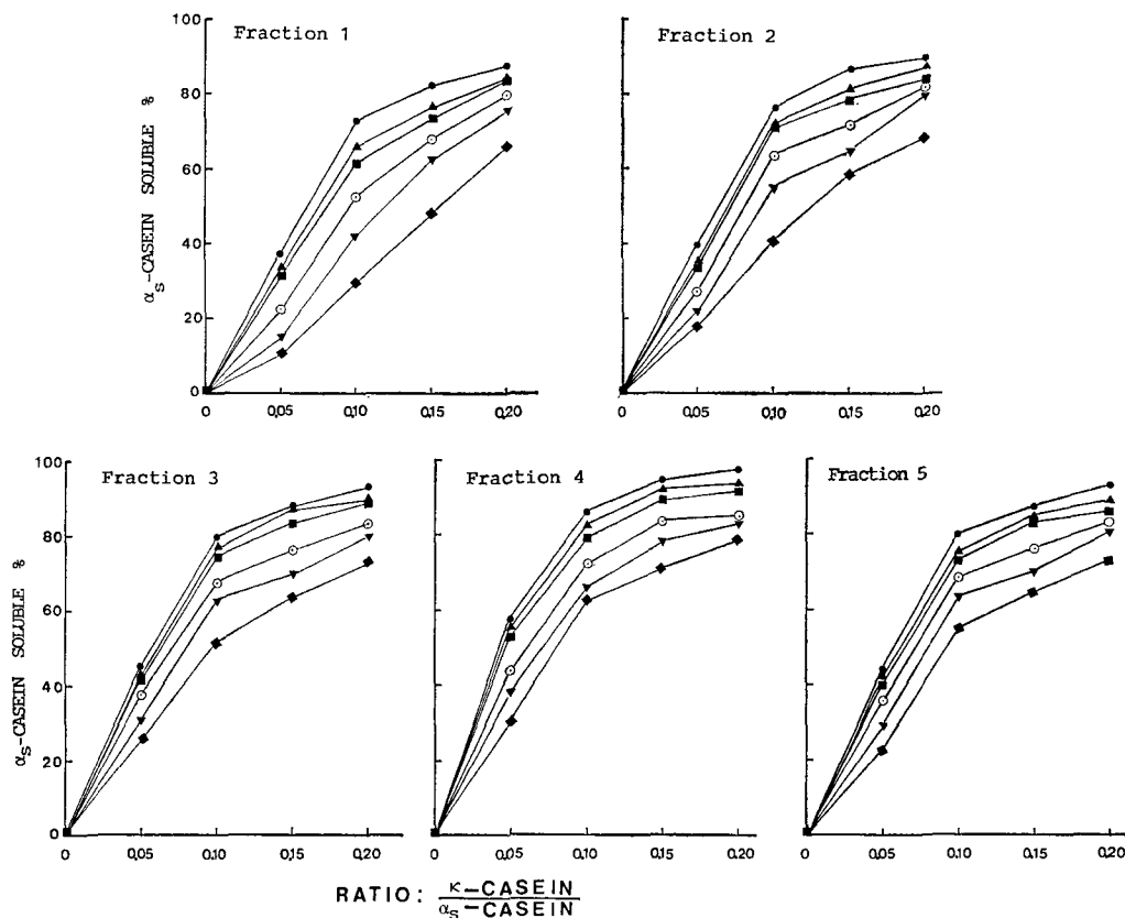
Fig. 4. Effect of heating for 5 min. on the ability of \kappa -casein fractions to stabilize \alpha_s -casein in the presence of 0.02 M \text{CaCl}_2 . Varying volumes of \kappa -casein fraction (0.5% w/v) were added to 1 ml of 1% (w/v) \alpha_s -casein followed by adding 1 ml 0.1 M \text{CaCl}_2 . Total volume of the test mixture was 5 ml.
