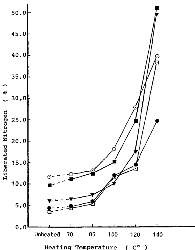
Fig. 3. Liberated N in pH 4.6-filtrate from \kappa -casein fractions by heating for 5 min.
