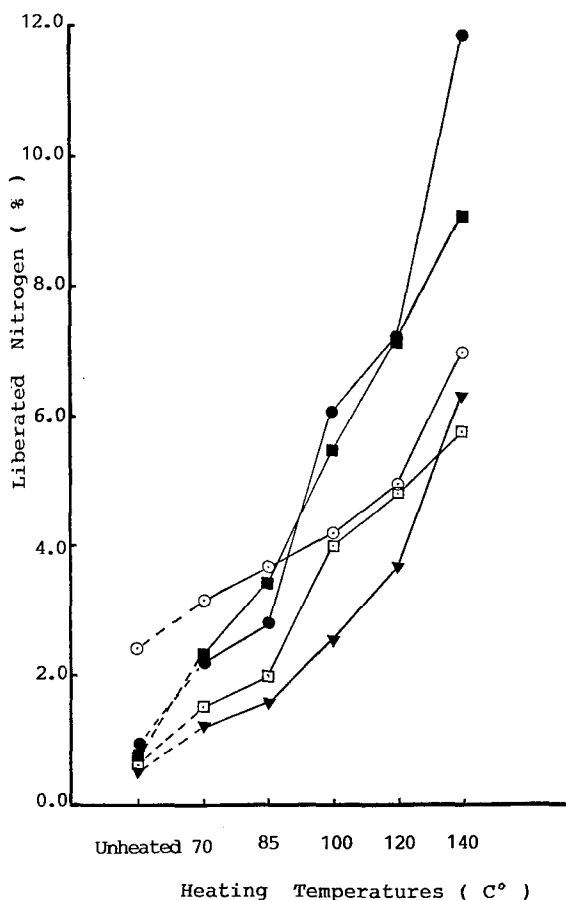
Fig. 2. Liberation of NPN from \kappa -casein fractions by heating for 5 min.
