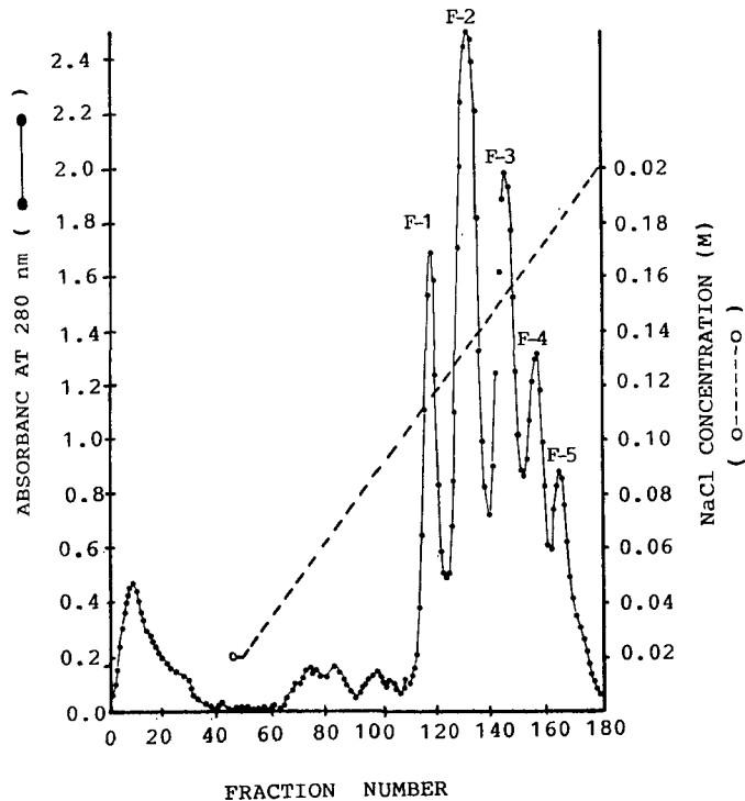
Fig. 1. DEAE-cellulose chromatographic pattern of \kappa -casein prepared by the modified urea-sulfuric acid method. 900 mg of \kappa -casein was dissolved in 45 ml of the starting buffer and reduced with 2-mercaptoethanol under nitrogen gas at 5°C for 16 hr. Reduced \kappa -casein was applied to a DEAE-cellulose column (4.5×20 cm). A flow rate was maintained at 85 ml per hr. One tube containing 10 ml.
