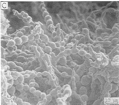
Fig. 11. Ambrosiella sp. isolated from the mycetangia of S. shogun . a. Ambrosiella sp. growing from the mycetangia of S. shogun on an agar plate. b. At higher magnification under the light microscope. c. d. Like chains under a scanning electron microscope.
