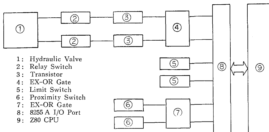
Fig. 7. Interface circuit used in the steering system.
