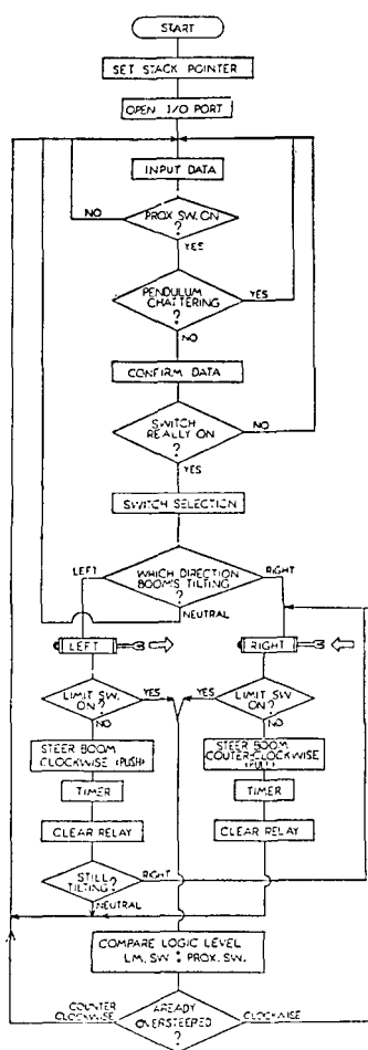
Fig. 8. Flow-chart of the control program used in the steering test. This program required about 1 kB of memory in machine language.
