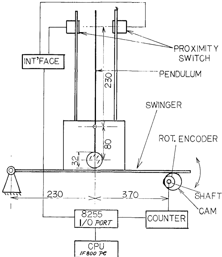
Fig. 1. Pendulum type inclinometer, sensitivity test stand and data acquisition system.
