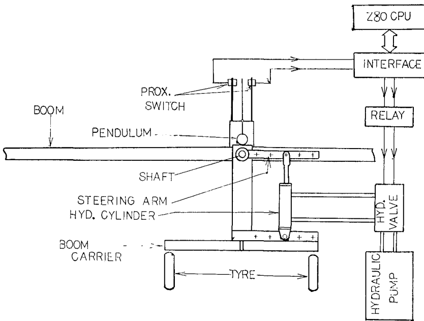
Fig. 6. Steering system. This steering system consists of a pendulum type inclinometer, a hydraulic actuator, and a computer-controlled control box.
