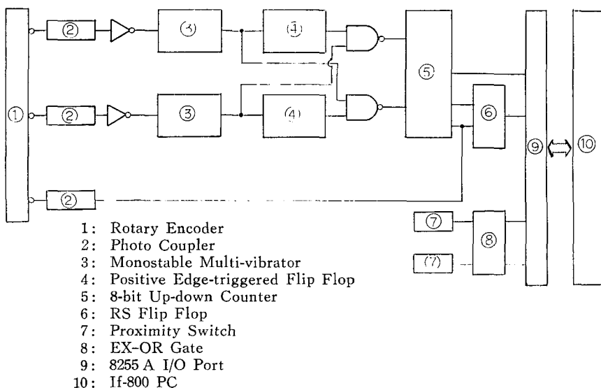
Fig. 2. Interface circuit used for the data acquisition in the sensitivity test of the inclinometer.
