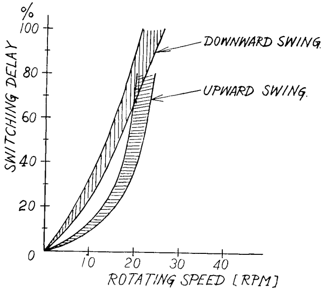
Fig. 5. Relationship between logic level transition delays of the proximity switches and the disturbance frequency.
