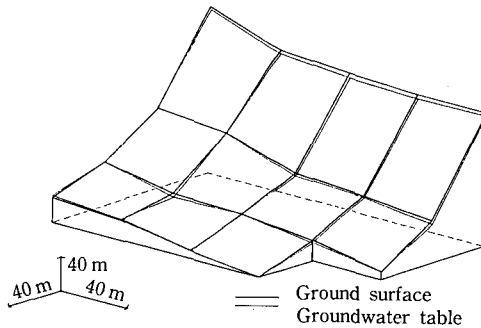
Fig. 2. Ground surface and groundwater table, Waqie.
