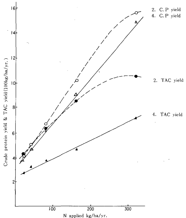
Fig. 5. Effect of N rate and cutting frequency on the crude protein yield and TAC yield in 6 orchardgrass varieties.
