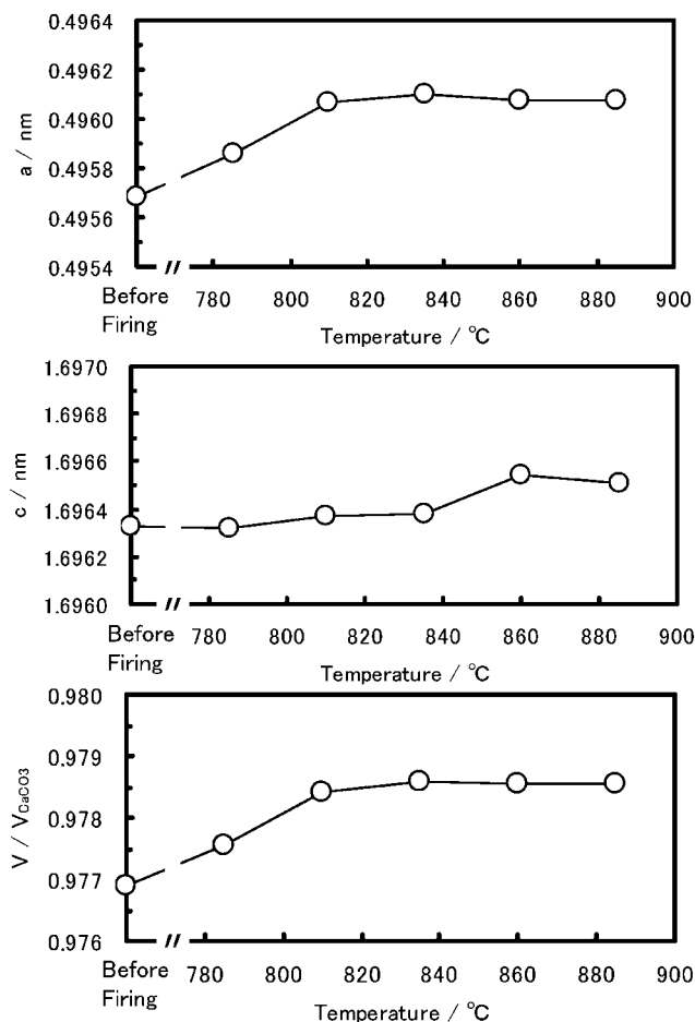
Fig. 5. Firing temperature dependence of the lattice parameters.
