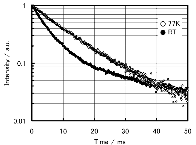
Fig. 12. Decay curves measured at room temperature and 77 K of the scallop shell fired at 835°C.
