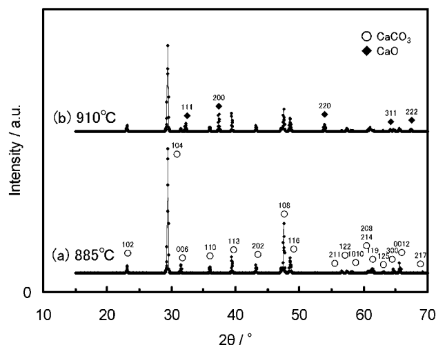
Fig. 4. Powder X-ray diffraction patterns of the scallop shells. (a): fired at 885^\circ\text{C} , (b): fired at 910^\circ\text{C} .
