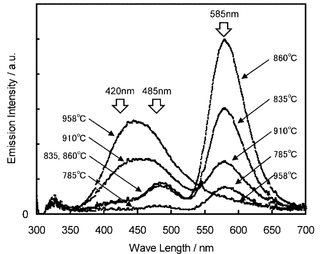
Fig. 8. Emission spectra of the scallop shells fired at various temperatures.
