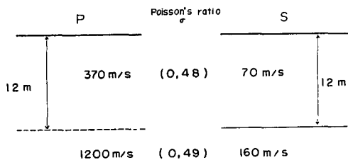
第8図 推定地下構造 Fig. 8. Subsurface structure deduced from S- and P-waves refraction at Wakino-machi.
