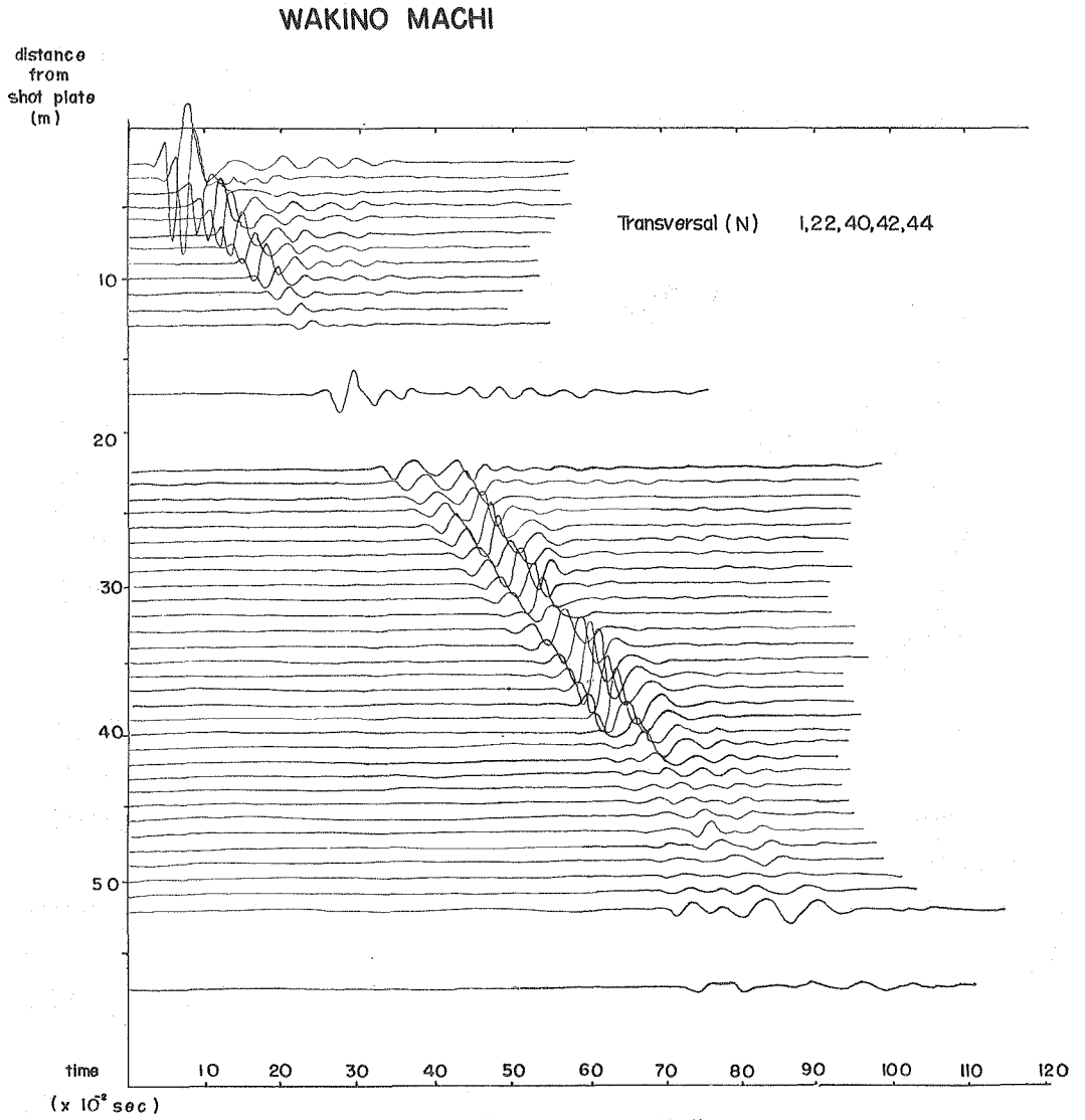
Fig. 4. Seismic records composed from five records at Wakino-machi.
