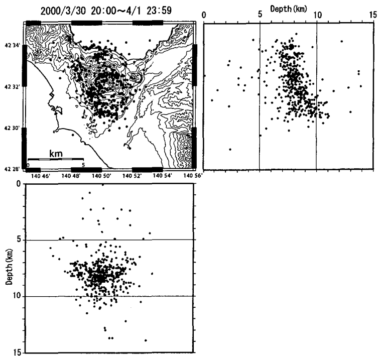
Fig. 6d. Hypocenter distribution. (2000/3/30 20:00 - 4/1 23:59)
