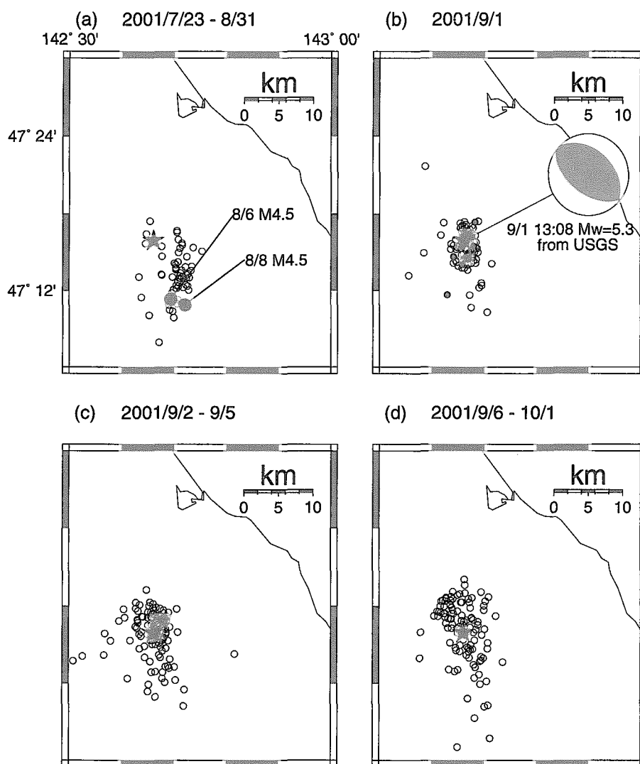
Fig. 10. Maps showing the spatial development of the swarm activity in the boxed area in Fig. 8. Star indicates the epicenter of the largest earthquake on September 1 ( M_w=5.3 ).
