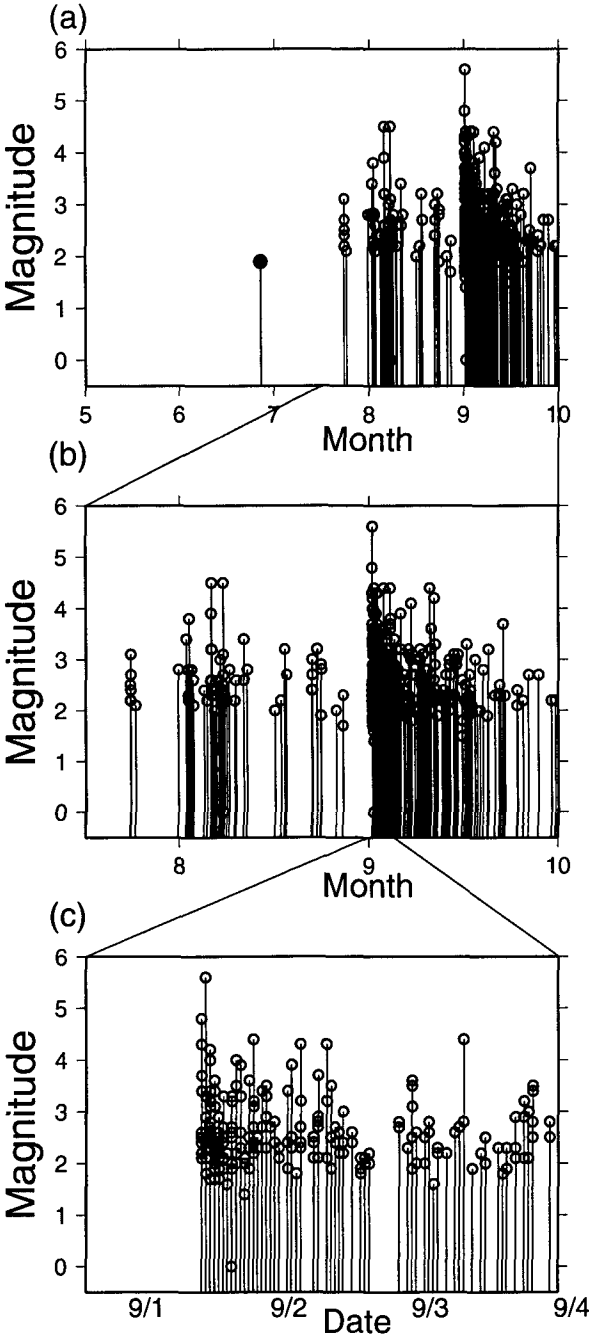
Fig. 9. Magnitude-time diagram of earthquakes obtained from the temporary seismic observation in 2001. (a) From May 1 to Sep. 30, 2001. Open circles indicate earthquakes in the swarm of 2001. Only three events (June 26, Aug. 2 and Sept. 17) are not included in the swarm. (b) Swarm activity in the boxed area of Fig. 8. (c) Swarm activity from September 1 to 4.
