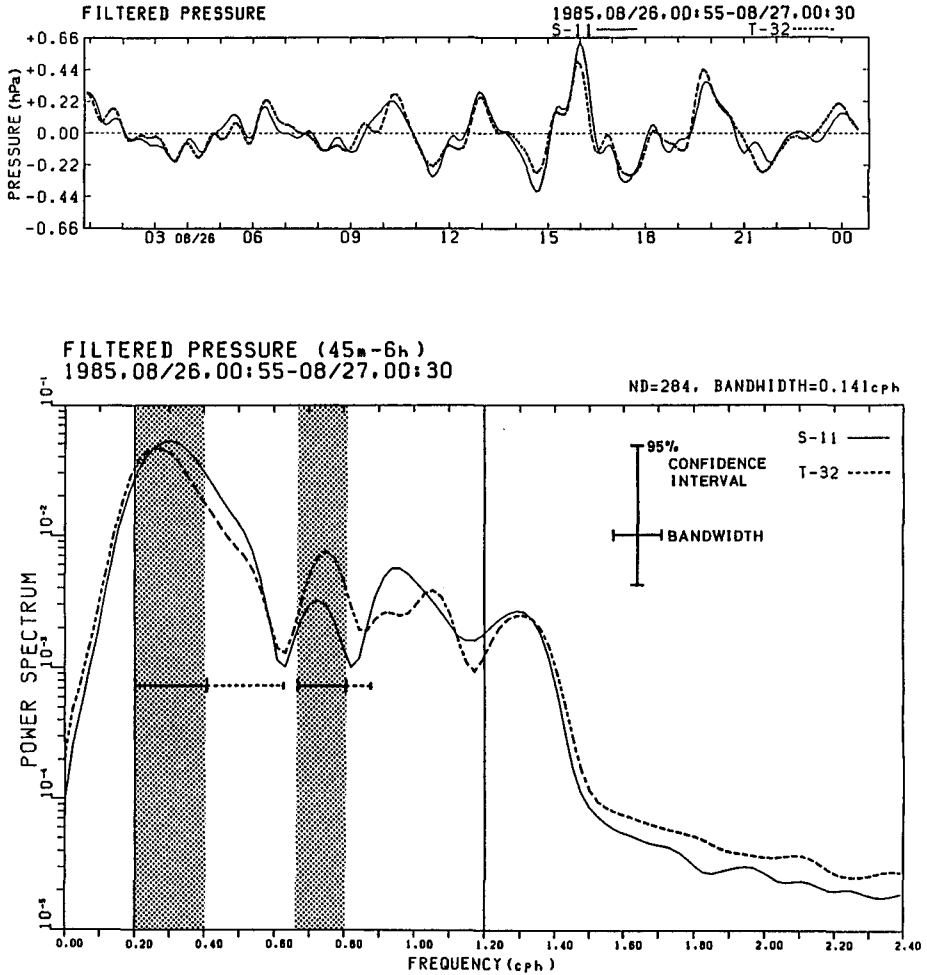
Fig. 7. Time series of perturbation pressure derived from the application of the first-step bandpass filter shown in Fig. 6 to pressure at the S-11 and T-32 sites (top) and the power spectra of the perturbation pressure shown in top panel (bottom). The solid and thick dashed lines correspond to the S-11 and T-32 data in both panels. See text.
