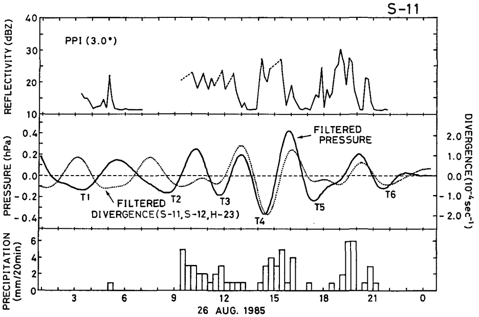
Fig. 10. Time series of reflectivity above S-11 on 3.0 degree PPI (top), perturbation pressure and surface divergence derived from the application of the second-step bandpass filter (middle), and rainfall intensity per 20 min (bottom) at S-11 site. Time series of the perturbation pressure and perturbation divergence are drawn by the solid and dotted line, respectively.
