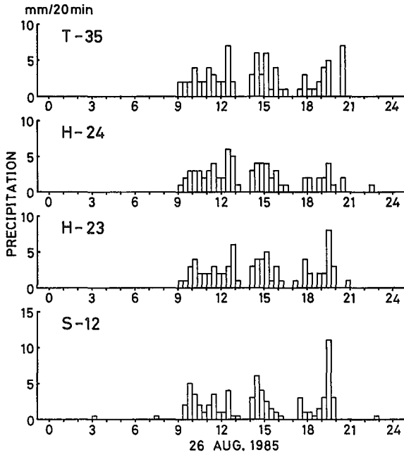
Fig. 4. Time series of rainfall intensity per 20 min at the sites of T-35, H-24, H-23 and S-12.
