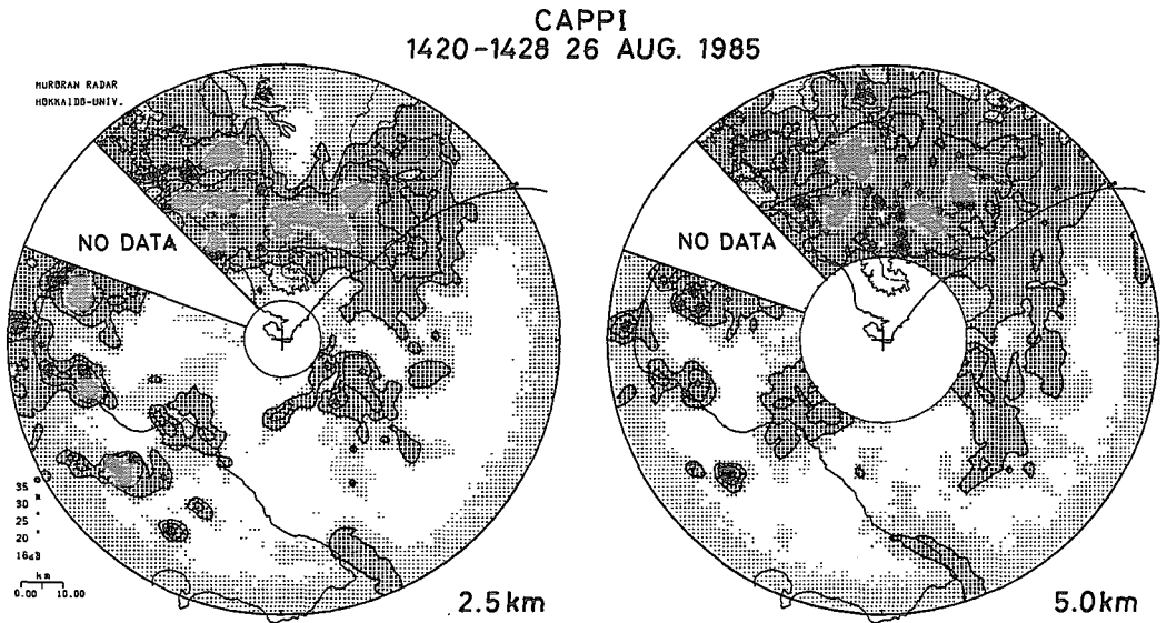
Fig. 5. CAPPI pictures at 2.5 km (left) and 5.0 km (right) a.s.l. for 14:20–14:28 JST on August 26, 1985. The echo intensities are indicated by both contours at 5 dBZ intervals from 20 dBZ and symbols shown on the lower left of the figure. The outer and inner circles of each panel show maximum range of 63.5 km and no data areas. The coastline, crestline and contours of 300 m a.s.l. are drawn by slightly thick solid, thin dashed and thin solid lines, respectively.
