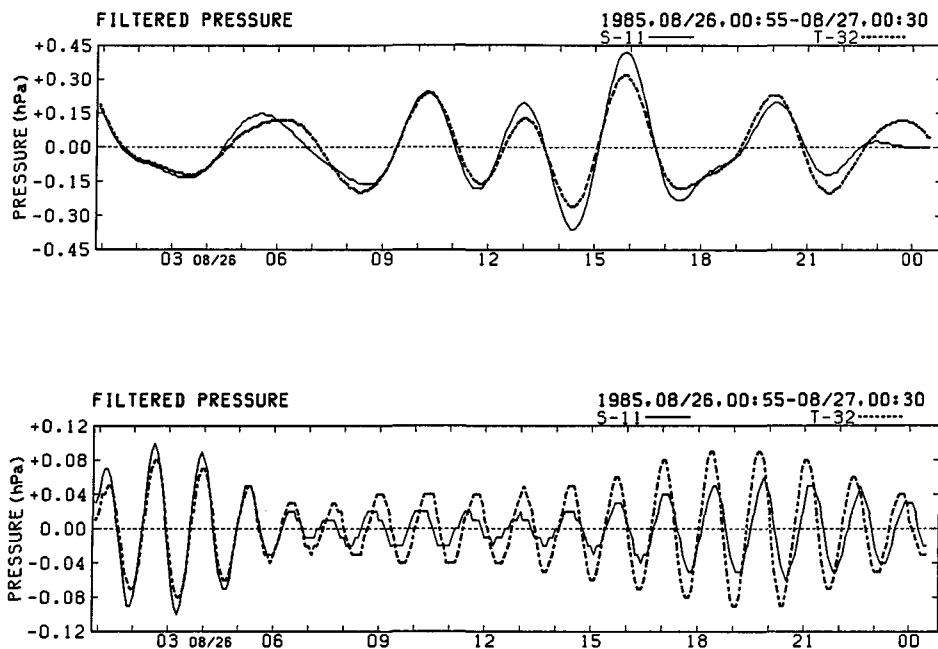
Fig. 8. Time series of perturbation pressure derived from application of two kinds of second-step bandpass filters to the S-11 (solid lines) and T-32 data (thick dashed lines).
