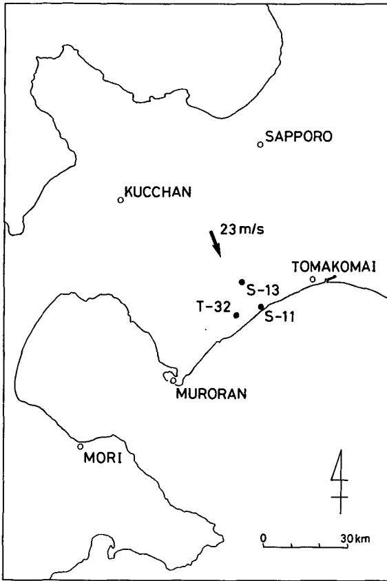
Fig. 11. Map of the surrounding barometer sites used for the phase velocity calculations. The solid and open circles indicate the locations of our microbarometer sites and meteorological observatories supported by JMA, respectively. The arrow shows the derived phase velocity of the observed gravity wave.
