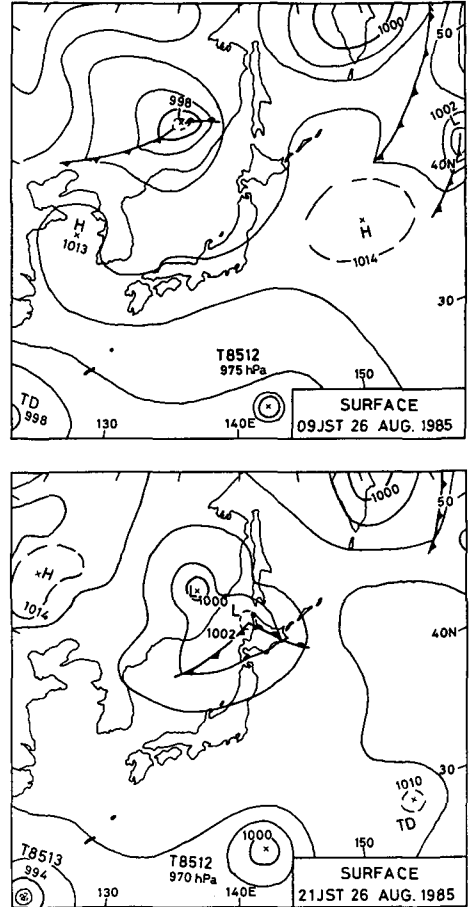
Fig. 2. Surface weather charts at 09 and 21 JST on August 26, 1985.
