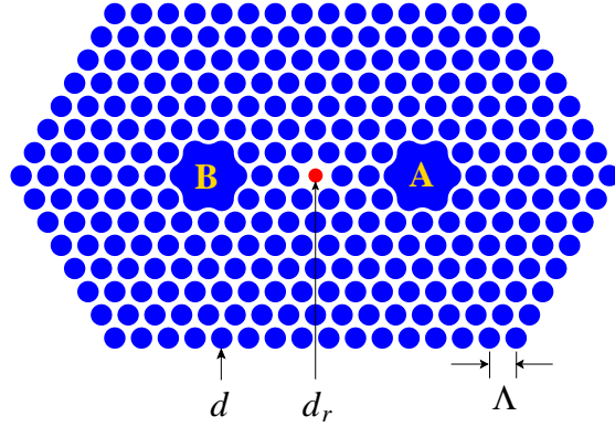
Fig. 9. Dual-core PBGF splitter with an embedded resonator in its profile, for achieving polarization-independent propagation characteristics.
