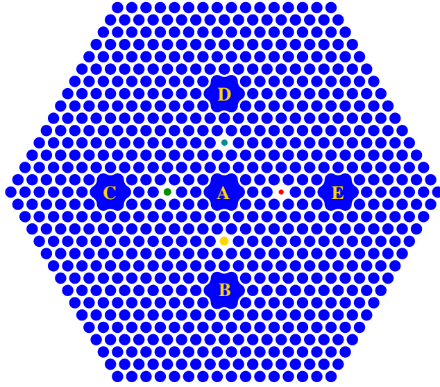
Fig. 11. Topology of the proposed five-core PBGF splitter utilizing a non-proximity resonant tunneling coupling mechanism. As an input core we consider the central core-A, while B, C, D and E are the output cores. Four dissimilar transverse resonators with diameters d_1 (yellow colored), d_2 (green colored), d_3 (teal colored), and d_4 (red colored) are introduced by reducing (high index defects) the diameters of the air-holes across the lines joining the cores. By a judicious choice of the design parameters this multicore PBGF can perform an ultra-narrow bandpass filtering operation at four distinct wavelengths with a reasonably short coupling length.
