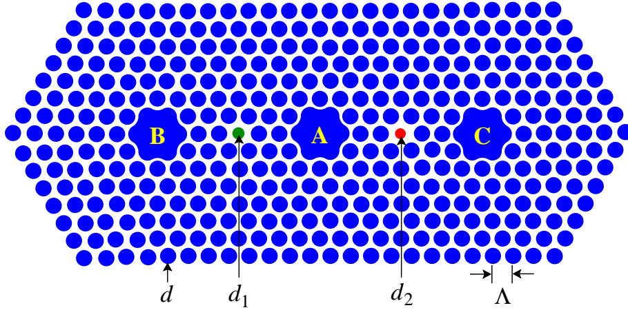
Fig. 1. Topology of a three-core PBG fiber splitter utilizing a non-proximity resonant tunneling coupling mechanism. The air-holes in the cladding are arranged in a triangular configuration with pitch constant \Lambda and air-hole diameters d . As an input core we consider the middle core-A, while B and C are the output cores. Two dissimilar transverse resonators with diameters d_1 (green colored) and d_2 (red colored) are then introduced by reducing (high index defects) the diameters of the air-holes in the middle of the line joining the cores. By a judicious choice of the design parameters this multicore PBGF can act as an ultra-narrow dual bandpass filter at a very short coupling length.
