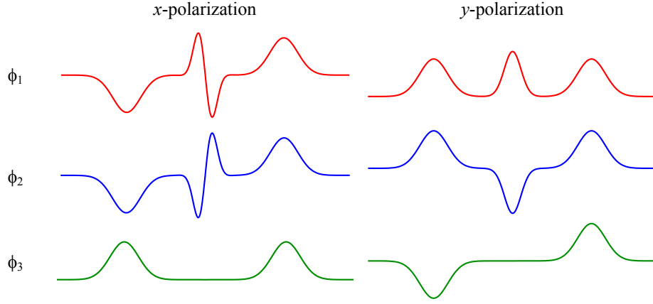
Fig. 4. Qualitative representation of the 3 supermodes existing in the MC-PBGF splitter.
