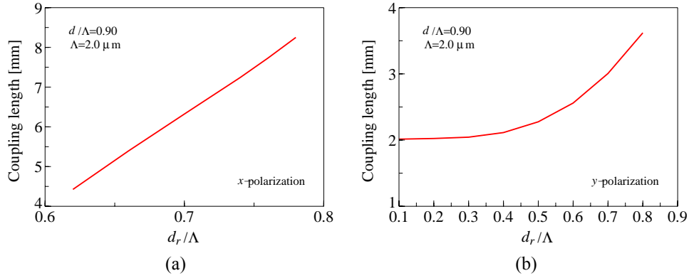
Fig. 5. Coupling length (mm) as a function of the normalized resonator's diameter d_r/\Lambda , for (a) x -polarization and (b) y -polarization. Observe the remarkable linear evolution of the curve in the case of x -polarization and the asymptotic behavior as the normalized diameter tends to lower values, for the y -polarization.
