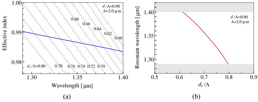
Fig. 2. (a) Effective indexes of the x -polarized fundamental (solid blue curve) and the x -polarized excited resonant modes (red dashed curves) of the multi-core PBG fiber splitter, for fixed design parameters d/\Lambda = 0.9 , \Lambda = 2 \mu\text{m} , and for several values of the normalized resonator's diameter d_r/\Lambda , ranged from 0.6 to 0.8, and (b) the evolution of the resonance wavelength as a function of the resonator's normalized diameter d_r/\Lambda . In this case the requirement that the resonance wavelength must lie within the PBG of the structure (between the grey boundaries), limits the normalized resonator's diameter d_r/\Lambda to vary from 0.62 up to 0.8.
