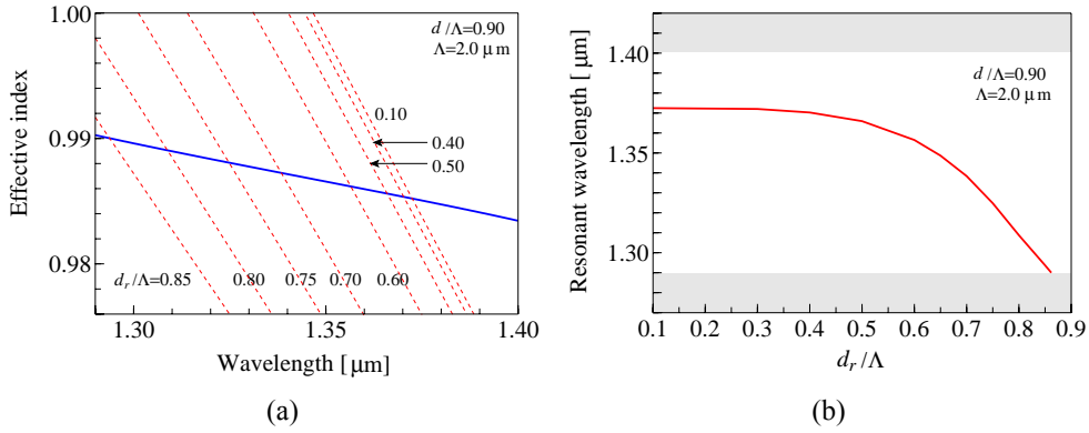
Fig. 3. (a) Effective indexes of the y -polarized fundamental (solid blue curve) and the y -polarized excited resonant modes (red dashed curves) of the multi-core PBG fiber splitter, for fixed design parameters d/\Lambda = 0.9 , \Lambda = 2 \mu\text{m} , and for several values of the normalized resonator's diameter d_r/\Lambda , ranged from 0.1 to 0.85, and (b) the evolution of the resonance wavelength as a function of the resonator's normalized diameter d_r/\Lambda . Notice the remarkable insensitivity in the evolution of the resonant wavelength as a function of the resonator's diameter in the range from 0.1 to 0.4 for the y -polarization. The PBG boundary is denoted within the grey strips.
