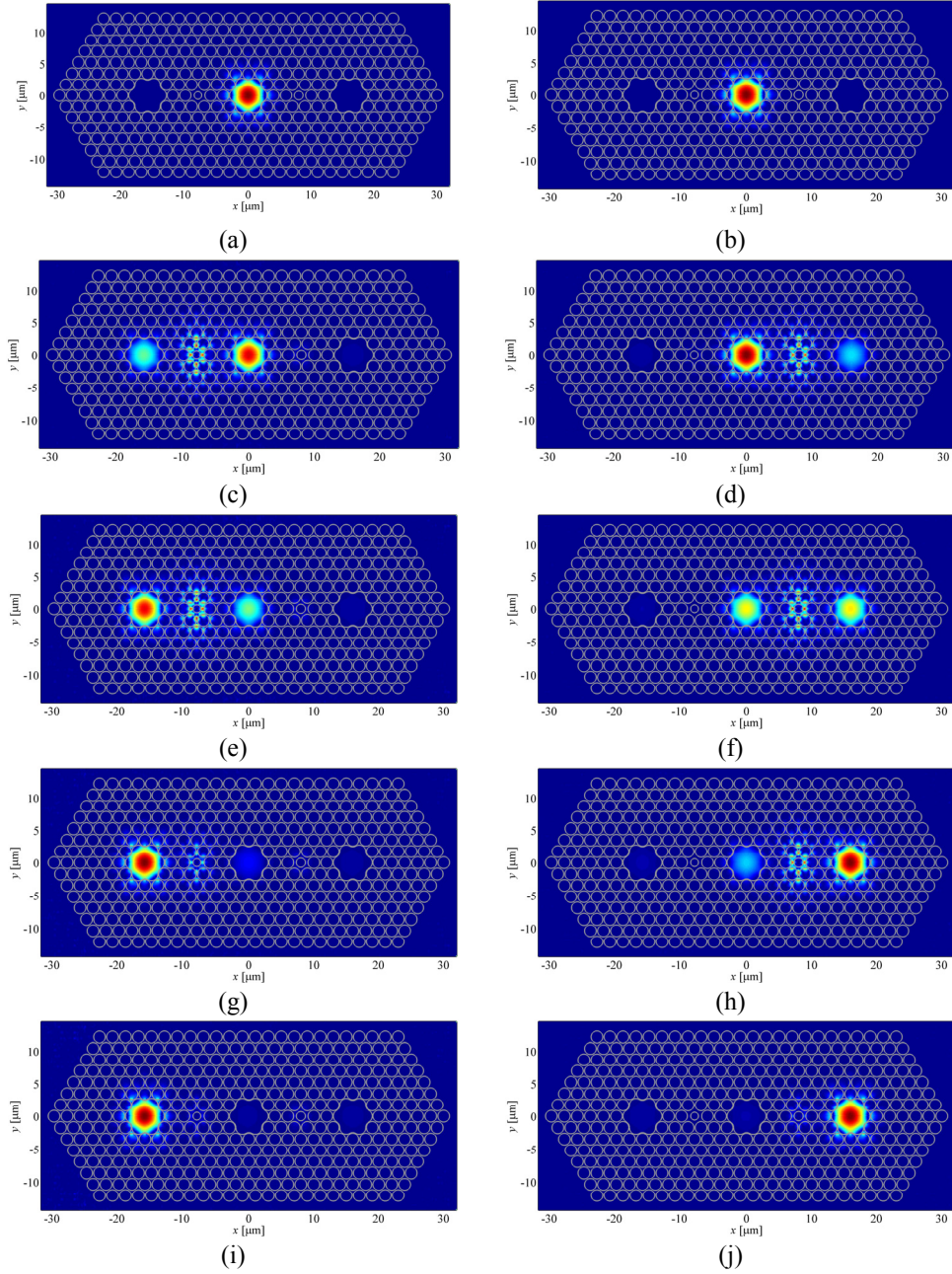
Fig. 7. Snapshots of the electric field distributions, that is y -polarization ( E_y ), in the multi-core PBGF splitter, for (a) \lambda_{1,y} = 1.339 \mu\text{m} , (b) \lambda_{2,y} = 1.357 \mu\text{m} , calculated at a distance of z = 0 mm, (c) \lambda_{1,y} = 1.339 \mu\text{m} (d) \lambda_{2,y} = 1.357 \mu\text{m} , at a distance of z = 1.0 mm, (e) \lambda_{1,y} = 1.339 \mu\text{m} , and (f) \lambda_{2,y} = 1.357 \mu\text{m} , at a distance of z = 1.5 mm, (g) \lambda_{1,y} = 1.339 \mu\text{m} , and (h) \lambda_{2,y} = 1.357 \mu\text{m} , at a distance of z = 2.0 mm, and finally for (i) \lambda_{1,y} = 1.339 \mu\text{m} , (j) \lambda_{2,y} = 1.357 \mu\text{m} , calculated at the coupling length of z = L_c = 2.7 mm. We can clearly see that at the coupling length of L_c = 2.7 mm, almost complete power transfer can be achieved from the input core-A to the output cores B and C at wavelengths of \lambda_{1,y} = 1.339 \mu\text{m} and \lambda_{2,y} = 1.357 \mu\text{m} , respectively with a transmission level of about 95 % due to the slightly difference in the values of the exact coupling lengths at the two different wavelengths.
