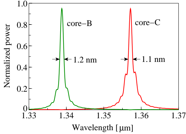
Fig. 6. Dual band-pass filtering characteristics for y -polarization of the three-core PBG fiber splitter, at the two resonant wavelengths of \lambda_1 = 1.339 \mu\text{m} and \lambda_2 = 1.357 \mu\text{m} , with corresponding full width at half maximum (FWHM) bandwidths of 1.2 nm and 1.1 nm, respectively. The transmission peak at the exact resonance wavelengths is about 95 % a result that indicates the slightly difference between the partial coupling lengths at the two different wavelengths.
