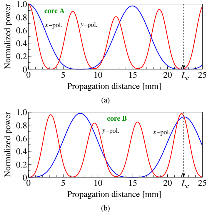
Fig. 10. Normalized power distribution in the MC-PBGF-splitter for x-polarization (blue curve), and y-polarization (red curve), at operating wavelength of \lambda_{\text{res}} = 1.325 \mu\text{m} , and for (a) input core-A, (b) output core-B. The coupling length for polarization-independent operation was confirmed by the BPM analysis to be L_c = 22.3 \text{ mm} . Thus by fixing the MC-PBGF splitter's length at the prescribed value, the structure operates as a dual-core coupler, with a transmittivity of more than 90 %, independent of the polarization state.
