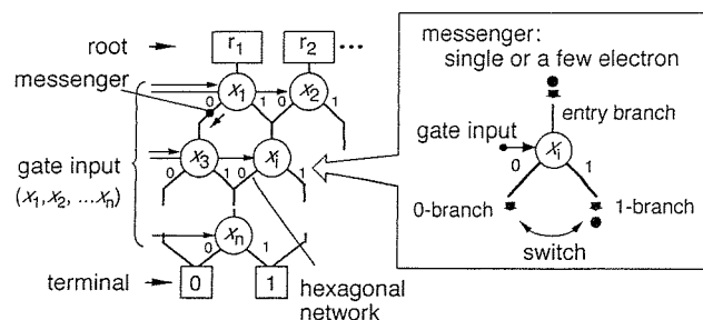
Fig. 4 Basic concept of the hexagonal BDD quantum logic circuit.
