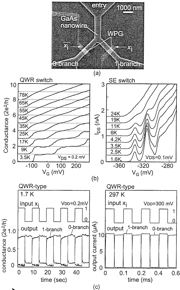
Fig. 6 (a) An SEM photograph of a QWR type BDD node device, (b) observed branch switch behavior of QWR- and SE-type BDD node devices and (c) path switching behavior of QWR-type node device at 1.7 K and room temperature.
