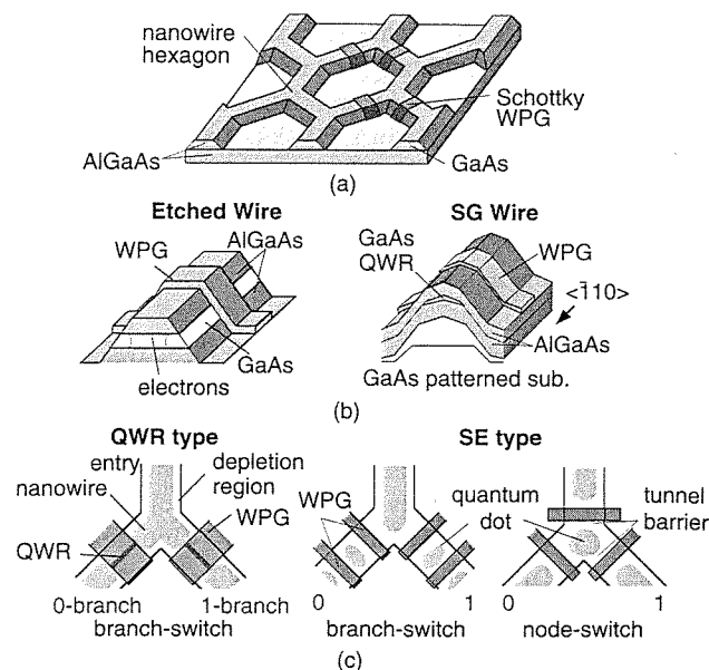
Fig. 5 GaAs-based implementation of BDD quantum node devices. (a) Circuit implementation by hexagonal nanowire network controlled by WPG, (b) basic structure of WPG and (c) WPG-based quantum BDD node devices.
