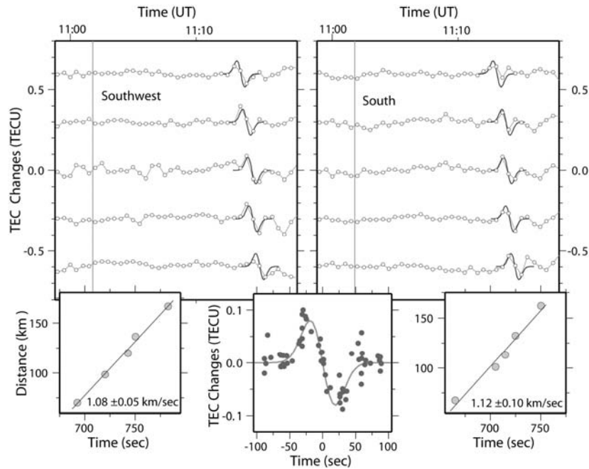
Figure 2. Arrival times of the disturbances are determined by searching for the time lag giving minimal differences between the source function (dark gray curves, see equation 1 of the text) and the observed TEC (open circles with the sampling interval of 30 seconds), for GPS points observing the southwestern (top left) and southern (top right) skies (Fig.1). Linear regressions are performed for the estimated arrival times (bottom left and right), and the apparent velocities of the disturbance propagation of \sim 1.1 km/s were estimated. Observed TEC values from the ten time series are compared with the source function after adjusting the time lags (bottom center).
