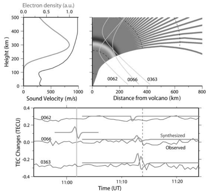
Figure 3. Relative electron density (light gray) and velocity of acoustic wave (dark gray) are plotted as functions of height [ Calais et al. , 1998] (top left). Ray tracing of acoustic waves for zenith angles 0-20 degrees is done assuming this velocity profile (top right). Equal-time contours are shown for 5, 10, 15, and 20 minutes after the eruption with broken curves. Gray scales shown along the ray paths indicate the position of the source function at 11.23 minutes after the eruption ( \sim 11:14 UT, broken line in the bottom panel). Gray curves are the line-of-sights connecting the satellites 15 and three GPS stations 0062, 0066, and 0363 (their positions shown in Fig. 1). They are straight in 3-dimensional space, but have apparent curvatures here because we took the distance from Asama as the horizontal axis. The observed (dark gray, residuals of the polynomial fit) and synthesized (light gray, based on the ray tracing) TEC time series of the three points for satellites 15 are given in the bottom panel. The observed arrival times, waveforms, and relative amplitudes are consistent with the synthesized curves for 0066 and 0363. Absence of signals in 0062 would be due to the directivity of ionospheric disturbances [ Heki and Ping , 2005].
