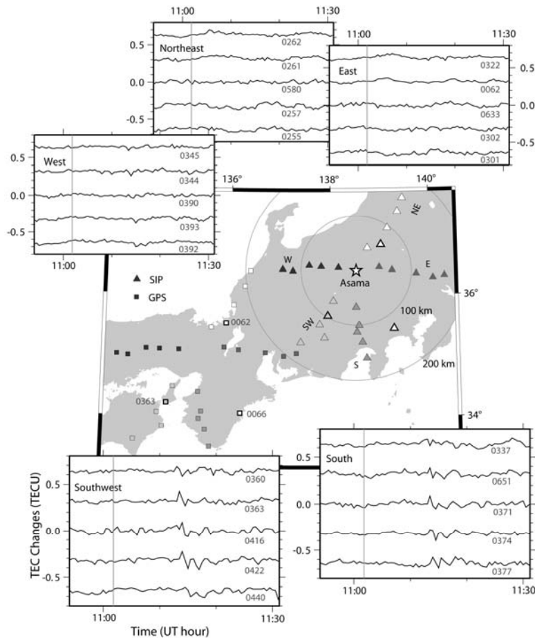
Figure 1. Time series of TEC (Sat.15) for GPS stations (squares) with the ground projections of the ionosphere (height is assumed to be 300 km) piercing points (triangles) in different azimuths from the volcano (open star). There are clear disturbances in southern and southwestern stations about 10 minutes after the eruption (11:02, vertical gray lines). They are less conspicuous in the western stations and absent in northeastern and eastern stations. Numbers in the time series are the station IDs in four digits. TEC time series closer to the volcano are displayed in upper positions. Time series of the three GPS stations shown by squares with bold frames (0062, 0066, and 0363) are compared with synthesized ones in Fig. 3.
