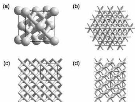
Figure 1. Model of the inverse opals with skeleton structure: (a) cubic unit cell with a lattice constant a ; (b) view towards (111) plane; (c) view towards (100) plane; (d) view towards (110) plane. In the model, the diameter of the tetrahedral and square prism vertexes was 0.12a and 0.31a, respectively, using Diamond Version 3.1a (copyright Crystal Impact GbR).
