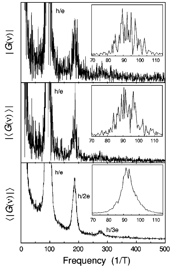
FIG. 3. The random features present in the modulus of the FS of a single magnetoconductance curve (upper graph) are not suppressed in the modulus of the FS of the averaged G(B) , |\langle G(\nu) \rangle| (middle graph). However, random features are clearly suppressed in the averaged modulus of the FS, \langle |G(\nu)| \rangle shown in the bottom graphs (in both the middle and in the bottom graphs, the average is taken over N = 49 curves measured at different gate voltages). Note the much enhanced visibility of the h/3e peak in \langle |G(\nu)| \rangle . The insets show the effect of sample specific features in the frequency range corresponding to the h/e peak. Also here the difference between the middle and bottom graphs is obvious and a splitting is clearly visible in the h/e peak of in \langle |G(\nu)| \rangle (note, in the main panel, that a small splitting is also present on top of the h/3e peak).
