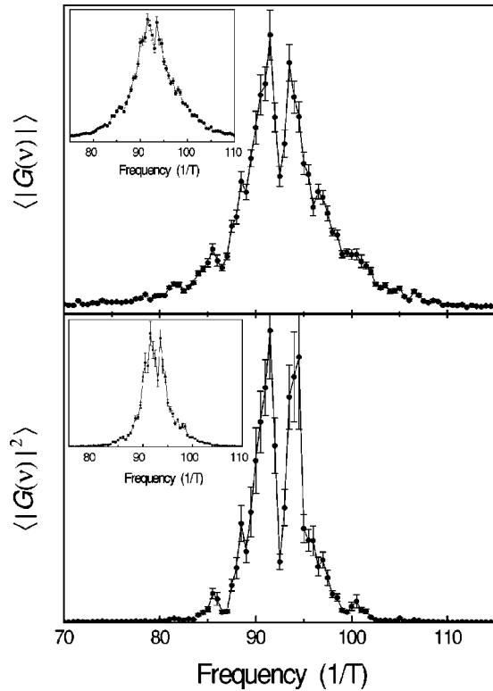
FIG. 4. The upper graph shows the h/e peak in the averaged modulus of the Fourier spectrum and the associated statistical error \sigma_{mean} . The average is performed over N=16 (main figure) and N=49 (inset) curves, measured at different V_g . The bottom graph shows the same statistical analysis for the power spectrum. The observed splittings are significantly larger than the corresponding \sigma and can therefore be discriminated from remnant sample specific features and attributed to a different physical phenomenon.
