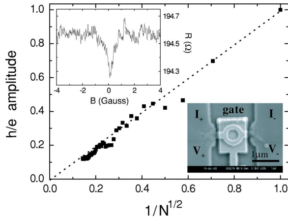
FIG. 2. Mean amplitude of the h/e oscillations in the averaged magnetoconductance, as a function of the square root of the number N of curves used in calculating the average. The mean amplitude of the h/e oscillations is calculated by integrating the modulus of the FS over the width of the h/e peak. The insets show the sample used in our investigations (bottom right) and the low-field magnetoresistance measured in a Hall bar made out of the same heterostructure used for our ring (top left). The resistance dip around zero field is due to weak antilocalization, which indicates the presence of strong Rashba spin-orbit interaction.
