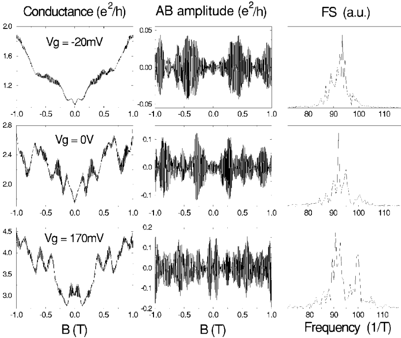
FIG. 1. The magnetoconductance of a ring measured at different gate voltage V_g at 300 mK is shown in the left column. The envelope function of the AB conductance oscillations, obtained by removing the positive magnetoconductance background, and the Fourier spectrum are shown in the middle and right column, respectively. It is apparent that both these quantities depend strongly on V_g , as it is typical for sample specific effects.
