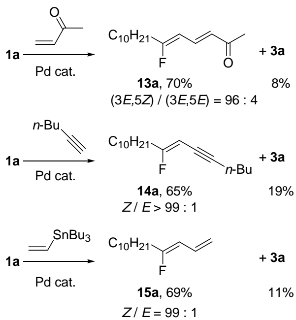
Scheme 1. Pd-catalyzed cross-coupling reactions using 1a
