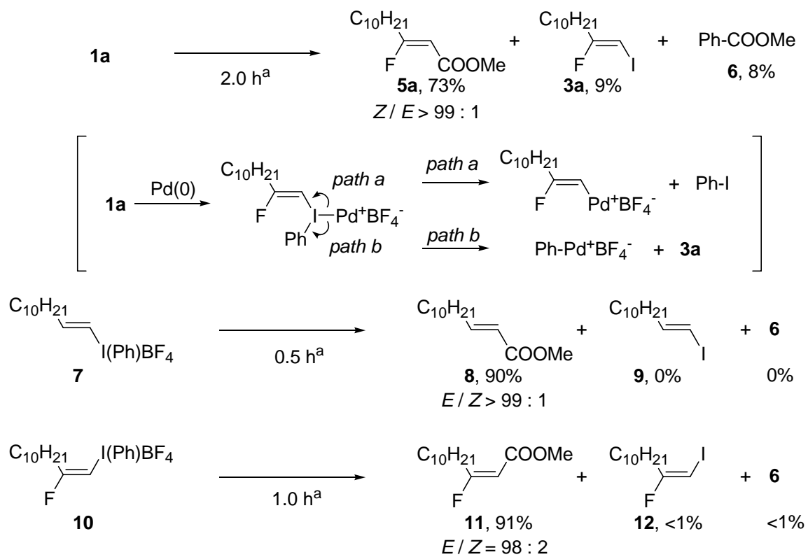
Figure 1. Methoxycarbonylation of 1a , 7 and 10
