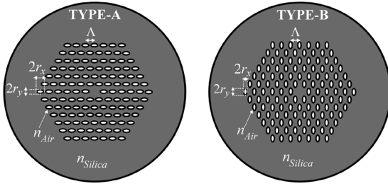
Fig. 1. Schematic cross section of the highly birefringent PCFs considered as polarimetric sensors, (left panel) type-A PCF with horizontally oriented elliptical air holes, and (right panel) type-B PCF with vertically oriented elliptical air holes.
