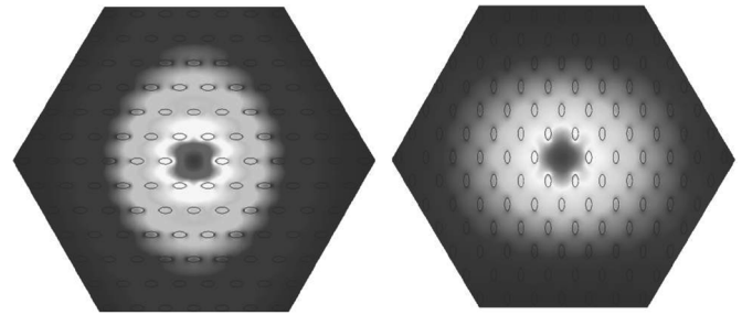
Fig. 4. Normalized intensity distributions of the fundamental mode calculated at maximum thermal sensitivity and for operational wavelength of \lambda = 1550 nm, for type-A PCF (left panel) and type-B PCF (right panel). The total number of air-hole rings is six for both cases.
