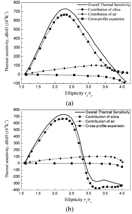
Fig. 2. Contributions of silica (circles), air (stars), and the cross profile expansion of the geometry (squares), to the overall thermal sensitivity ( \text{K}^{-1} ), at \lambda = 1550 nm, as a function of the air-hole ellipticity- e for (a) type-A PCF and (b) type-B PCF. For both cases, the maximization of the sensitivity function occurs for an air-hole ellipticity value of e = 2.27 .
