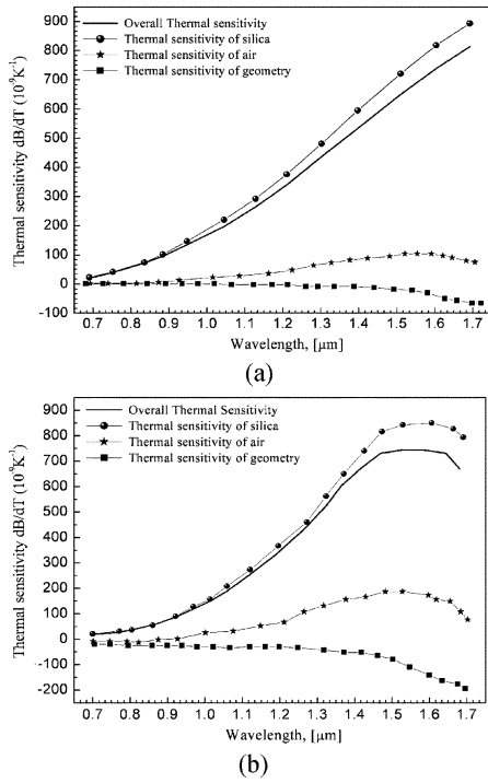
Fig. 3. Thermal sensitivity of the modal birefringence ( K^{-1} ) of silica (circles), air (stars), and the cross profile expansion of the geometry (squares), as a function of the operational wavelength \lambda in ( \mu m ), for (a) type-A PCF and (b) type-B PCF at fixed ellipticity of e = 2.27 .
