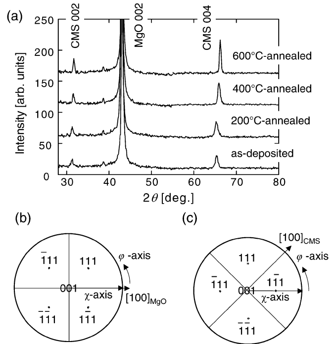
Fig. 2. (a) X-ray \theta - 2\theta diffraction patterns of 50-nm-thick CMS films as-deposited and postdeposition annealed at 200– 600^\circ\text{C} . (b) and (c) X-ray pole figures of (b) \text{MgO} 111 and (c) CMS 111 for a CMS film annealed at 600^\circ\text{C} .
